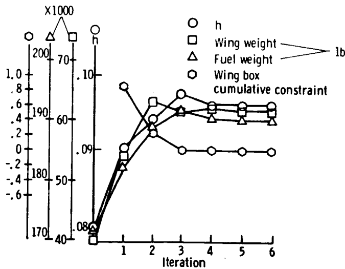
Figure 20. Histogram of an aircraft multilevel optimization.
