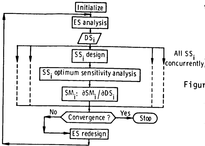
Figure 18. Two-level system optimization procedure.
