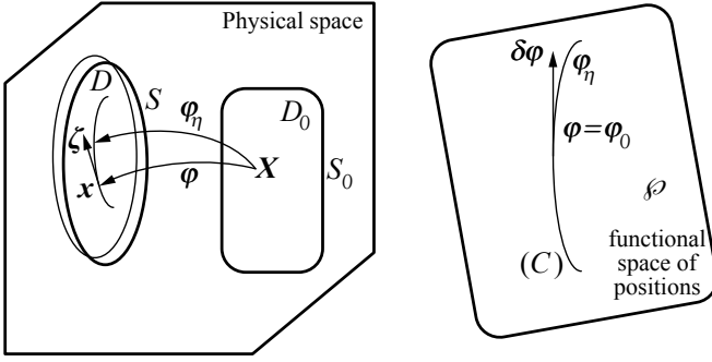
Figure 1. The boundary S of D is represented by a thick curve and its variation by a thin curve. The variation \delta\varphi of the family \{\varphi_\eta\} of varied paths belongs to T_\varphi(\wp) , tangent space of \wp at \varphi .
