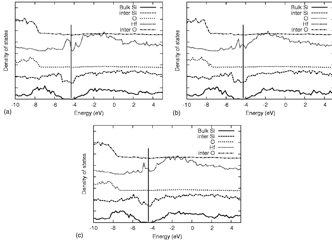
FIG. 10. PDOS for \text{HfO}_2 with an oxygen vacancy at positions (a) A, (b) B, and (c) C in Fig. 4.
