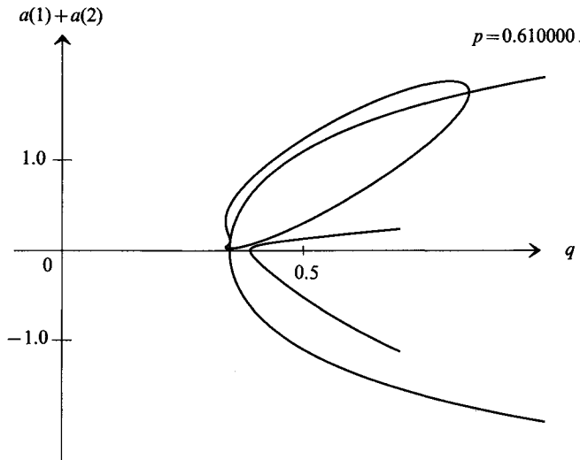
FIGURE 1. Bifurcation diagram when b = 1, \eta_1 = \eta_2 = 0 and p = 0.61 . q is taken as a bifurcation parameter. The y -axis represents the sum of the first two Fourier coefficients of \theta . A big loop having two turning points are observed.
