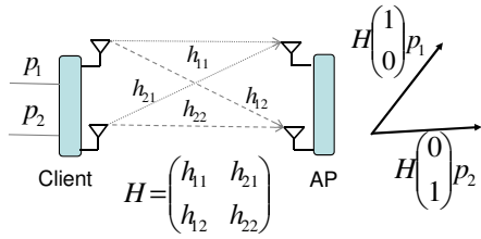
Figure 3: Two Packets on Uplink. The client transmits two packets, p_1 and p_2 , from its two antennas. The packets arrive along the vectors H[1\ 0]^T and H[0\ 1]^T , where H is the channel matrix and [\cdot]^T refers to the transpose of a vector. To decode p_1 and p_2 , the AP projects along the vectors orthogonal to H[0\ 1]^T and H[1\ 0]^T respectively.
