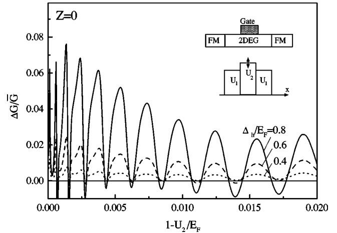
FIG. 4. \Delta G/\bar{G} of a two-dimensional transistor structure as a function of the Fermi energy below the gate electrode for various exchange energies for Z=0 . The inset shows the device structure.
