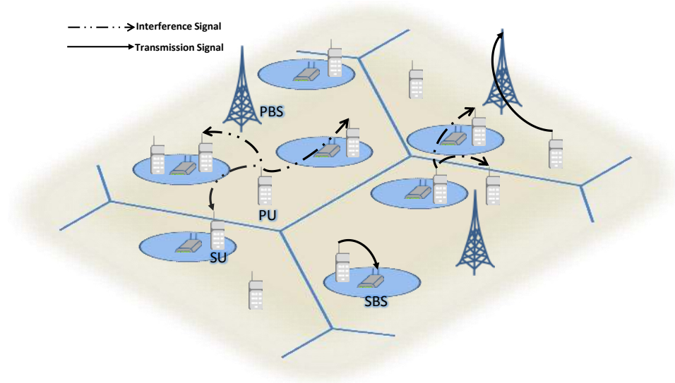
Figure 1.1 Heterogeneous network structure with SUs, PUs, SBSs and PBSs.
