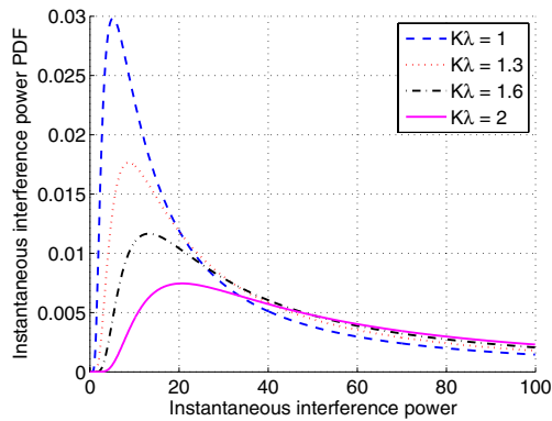
Fig. 2. Mean interference power PDFs without interference region ( R = 0 ).
