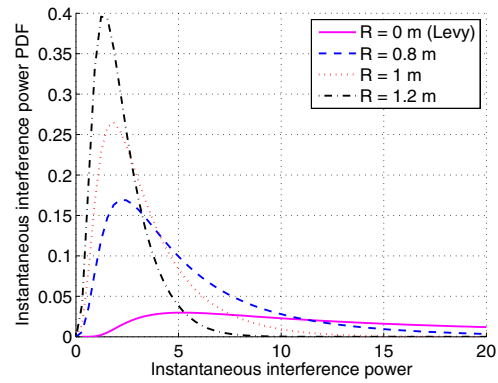
Fig. 5. Instantaneous interference power PDFs with an interference region ( \lambda = 1 , \sigma_s = 8 dB, and m = 1 ).
