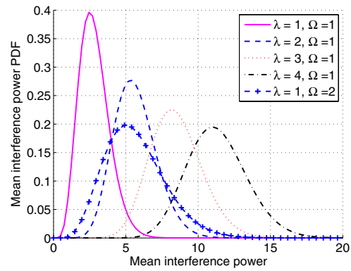
Fig. 4. Mean interference power PDFs with an interference region ( R = 1 m).
