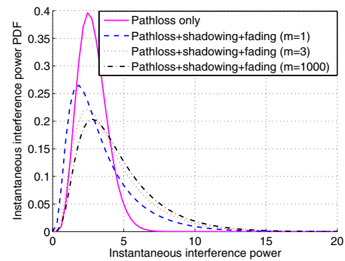
Fig. 6. Instantaneous interference power PDFs with an interference region under different fading scenarios ( R = 1 m, \lambda = 1 , and \sigma_s = 8 dB).
