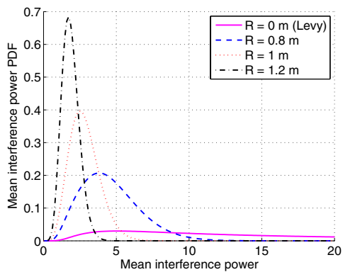
Fig. 3. Mean interference power PDFs with an interference region ( \Omega = 1 and \lambda = 1 ).
