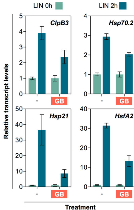
Fig 8. Pre-treatment with a chemical chaperone desensitizes the molecular response to LIN. Quantitative (qPCR) analysis of transcript levels of the indicated genes in 7-day-old WT plants grown in the presence or absence of glycine betaine (GB) and then transferred for 2h to fresh medium supplemented with 400 \mu M LIN. Data correspond to the mean and SEM values of n = 3 independent experiments and they are represented relative to the levels before the LIN treatment. For all the genes tested, statistically significant differences ( t test: p < 0.05 ) were found between the LIN-triggered induction of control and GB-grown samples.
