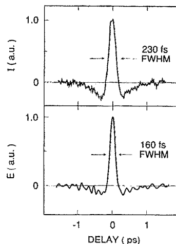
FIG. 2. (top) Interferogram of far-infrared light emitted from InP wafer. A constant offset has been subtracted as described in the text. (bottom) Inferred symmetric electric field E(t) derived from top.
