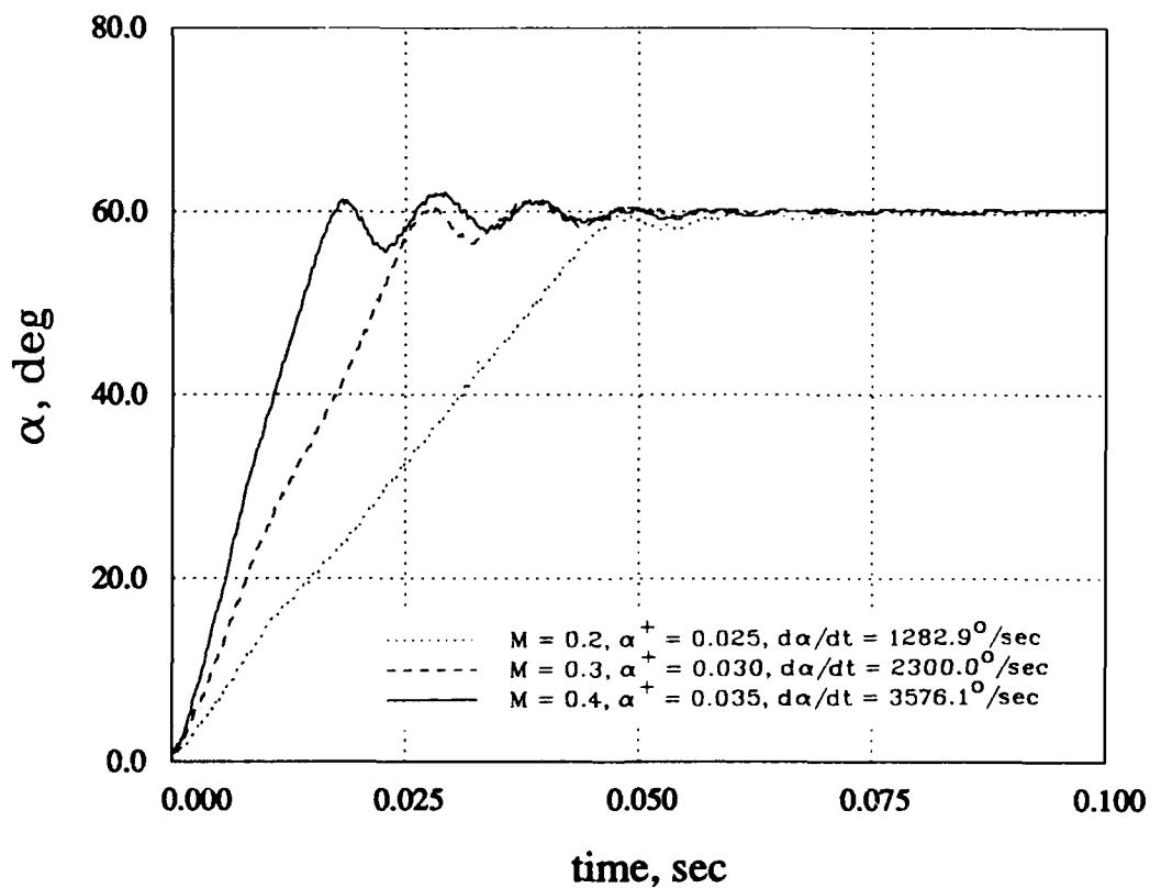
Fig. 2. Time History of Pitching Airfoil.
