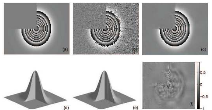
Fig. 4. Truncated Gaussian surface observed under independent but spatially variant Gaussian noise: the noise standard deviation varies linearly along the left-right directions from 0.3 to 0.9. Top and from left to right: true, noisy, and SpInPHASE estimate using the learned dictionary. Bottom and from the left to the right: true phase, unwrapped phase, and the SpInPHASE interferometric error \hat{\phi}_{2\pi} - \phi_{2\pi} .
