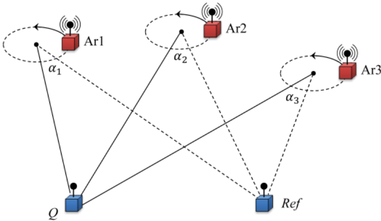
Fig. 11. Localization based on bearing estimates towards rotating transmitter nodes.
