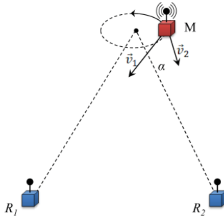
Fig. 9. Estimation of the angle between two receivers and a rotating anchor node.
