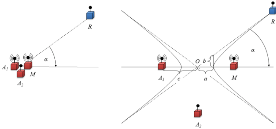
(a) Relative bearing from the 3-node anchor (b) The 3-node anchor exaggerated to show distances
