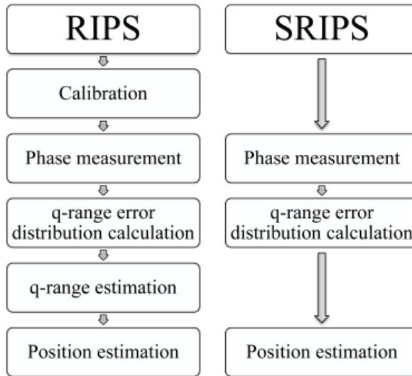
Fig. 13. Comparison of the original (RIPS) and the stochastic interferometric localization algorithms
