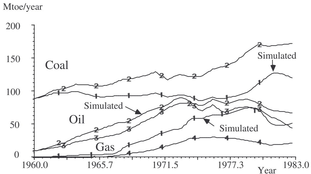
Figure 4: Historical and simulated development of the demand for coal, oil and gas; no premiums and no flexibility. Source for historical data: OECD Energy Balances.
