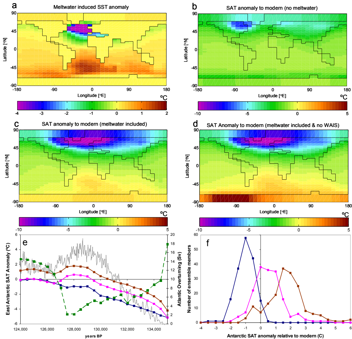
Fig. 4. GENIE-1 ensemble-averaged SST and SAT anomalies. Fields (at 128 500 BP) of (a) meltwater induced SST anomaly ( E_{FW}-E_{NFW} ) and (b, c, d) SAT anomalies relative to an equilibrium preindustrial ensemble E_{PI} with (b) no meltwater flux ( E_{NFW}-E_{PI} ), (c) including Laurentide and Eurasian meltwater fluxes ( E_{FW}-E_{PI} ) and (d) including Laurentide and Eurasian meltwater fluxes and replacing West Antarctic Ice Sheet with land at sea-level ( E_{WAIS}-E_{PI} ). (e) Ensemble-averaged temporal behaviour of East Antarctic SAT anomaly. The dashed green line is the ensemble-averaged ( E_{FW} ) Atlantic overturning (maximum streamfunction at depths below 400 m). The grey line is the DOME C deuterium inferred anomaly (Jouzel et al., 2007). Solid lines are East Antarctic SAT anomalies with blue: no meltwater forcing ( E_{NFW}-E_{PI} ), pink: meltwater forcing included ( E_{FW}-E_{PI} ), brown: meltwater forcing included and WAIS removed to land at sea level ( E_{WAIS}-E_{PI} ). (f) Ensemble distributions of East Antarctic SAT anomaly at 128 500 BP.
