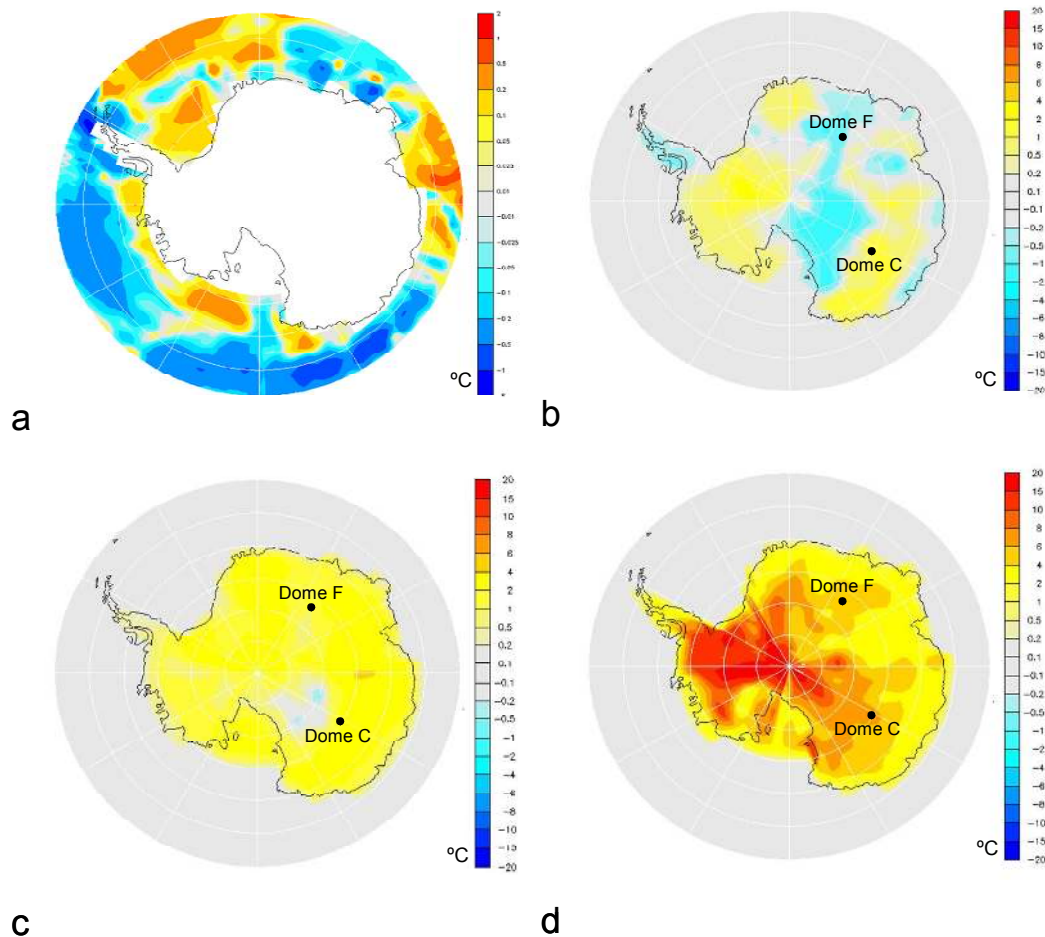
Fig. 5. HadCM3 SST and SAT anomalies at 130 000 BP. (a) Southern summer freshwater-induced SST anomaly due to 1 Sv North Atlantic hosing applied uniformly between 50–70° N ( H_{FW}-H_{NFW} ). (b, c, d) Precipitation-weighted SAT anomalies relative to preindustrial (b) with no hosing ( H_{NFW}-H_{PI} ), (c) including hosing ( H_{FW}-H_{PI} ), (d) including hosing and with WAIS removed to land at 200 m ( H_{WAIS}-H_{PI} ).
