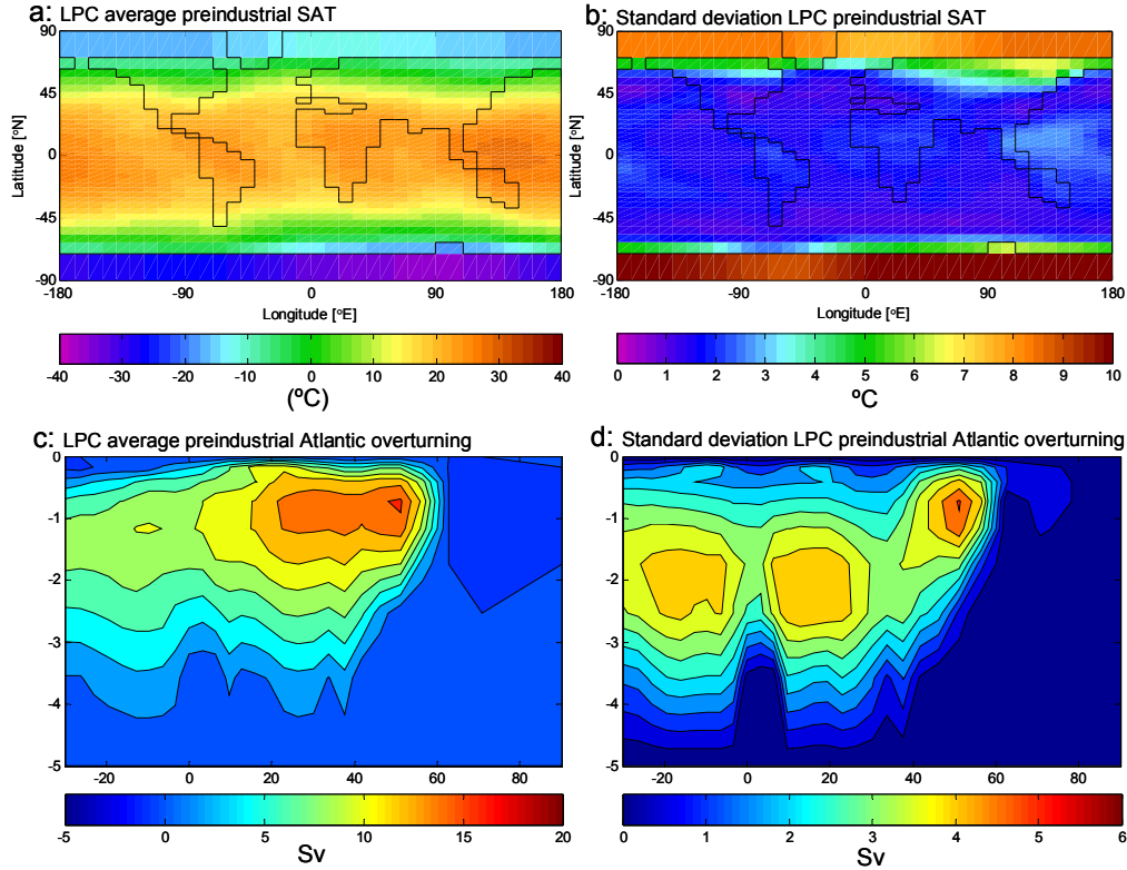
Fig. 2. Ensemble average and standard deviation of preindustrial (a, b) SAT (°C) and (c, d) Atlantic overturning stream function (Sv). Data are derived from the LPC (LGM Plausibility Constrained) parameter set (Holden et al., 2010).
