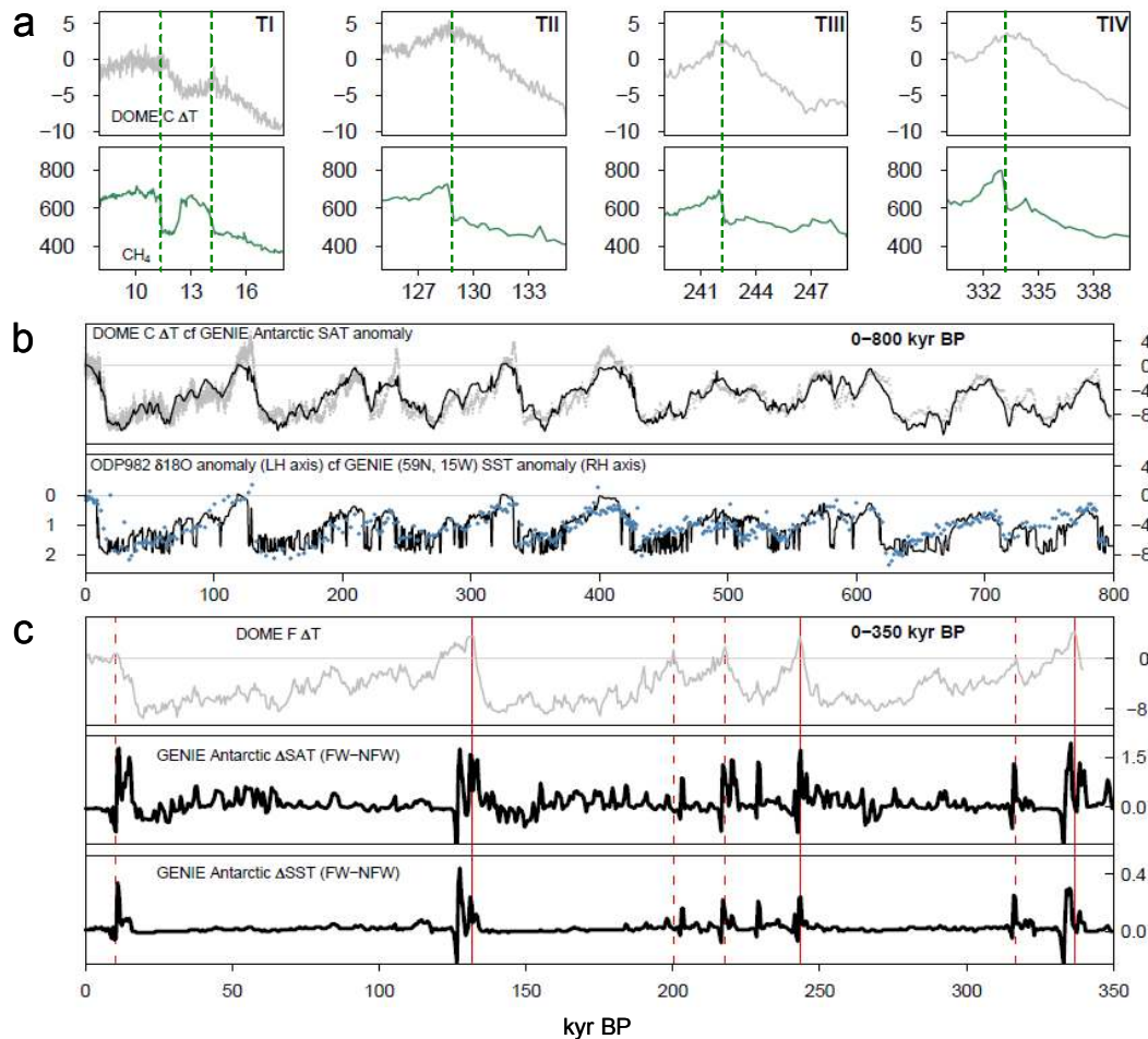
Fig. 1. (a) DOME C \delta D -inferred Antarctic temperature anomaly (Jouzel et al., 2007) (grey) and atmospheric CH_4 concentration (Loulergue et al., 2008) (green) at the last four terminations. (b) 800 kyr records of DOME C Antarctic temperature anomaly (grey) and planktonic \delta^{18}O anomaly (blue) at ODP site 982 (57.3° N, 15.5° W) (Venz et al., 1999), compared respectively with the GENIE-1 ( G_{FW} ) Antarctic SAT anomaly and the SST anomaly at the grid cell centred on 59° N, 15° W. (c) 350 kyr records of DOME F \delta D -inferred Antarctic temperature anomaly (Kawamura et al., 2007) (grey), GENIE-1 meltwater-induced ( G_{FW}-G_{NFW} ) Antarctic SAT and SST anomalies. SAT is averaged over Antarctica south of 71° S. SST is averaged over all the Southern Ocean south of 62° S. Note: the simulation in (b) includes meltwater forcing, but the effects in Antarctica (up to \sim 1.5^\circ C warming) are largely obscured by the larger changes across the terminations.
