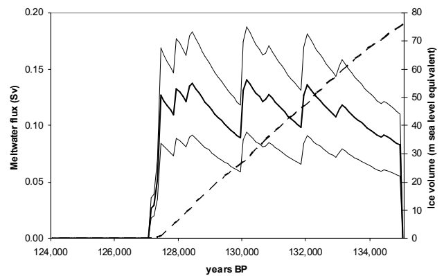
Fig. 3. Representation of ice sheets in the TII ensembles. The global distribution of ice sheets is given by Equation 1, assuming a constant reduction of \delta^{18}\text{O} from 4.86 to 3.16‰ from 135 000 to 126 000 BP. Meltwater is calculated at each grid cell and routed to the ocean assuming modern day topography. The dashed line illustrates total Laurentide and Eurasian ice sheet volume, expressed in equivalent meters of sea-level. The solid lines illustrates the profile of ensemble mean meltwater flux (bold, FFX = 1.5) and the range of meltwater fluxes (FFX = 1.0 to FFX = 2.0). The temporal development of meltwater is fixed across all ensemble members.
