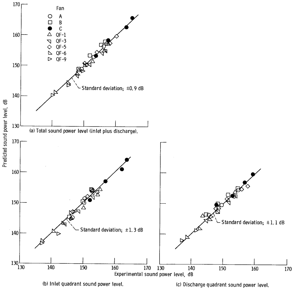
Figure 17. - Comparison of predicted and experimental sound power levels for NASA Lewis full-scale fans.
