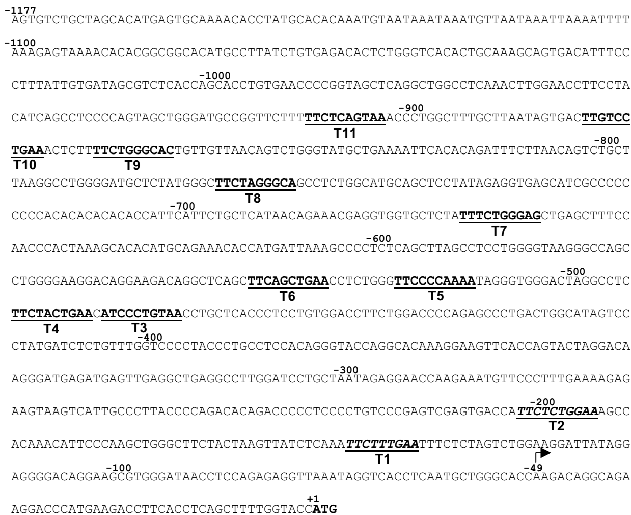
Figure 3 -1173 bp mTARC promoter and putative STAT6 sites. Sequence of the MDC-Fractalkine-TARC locus on mouse chromosome 8 was obtained from the Celera database and verified using the Sanger Centre database. Putative STAT6 sites in the proximal mTARC promoter were identified using low stringency searches using Genomatix MatInspector Release Professional 6.1 (November 2002) and the Transcription Element Search System (TESS). Sites conserved between human and mouse are written in italics. ATG indicates translation start codon, arrow indicates transcription start site and sequence positions are indicated as superscript, the start point of transcription of the mTARC gene as denoted + 1 [30].
