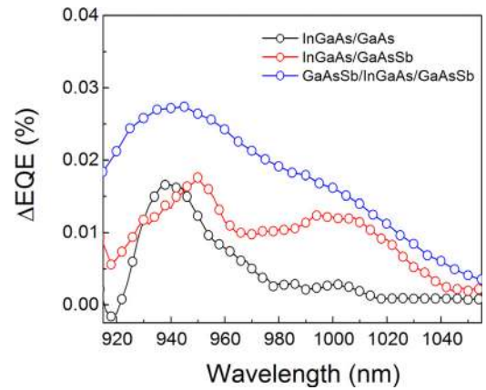
FIG. 38. Difference in EQE values, \Delta\text{EQE} , with ( \text{EQE}_{w/ \text{IR}} ) and without ( \text{EQE}_{w/o \text{IR}} ) IR light illumination.
