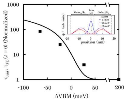
FIG. 35. Comparison for calculated \tau_{rad} (solid line) vs. experimentally determined PL decay time \tau_{PL}(t=0) (squares) at 77 K under weak excitation of 38 \text{ mW/cm}^2 . \Delta VB_M = -65 , -23 , and 27 meV correspond to the Sb compositions of 18%, 14%, and 10%, respectively. The lifetime is normalized by the value for the sample without Sb. Inset illustrates the magnitude of hole existence probability. Reprinted with permission from Nishikawa et al. , J. Appl. Phys. 111 , 044325 (2012). Copyright 2012 AIP Publishing LLC.
