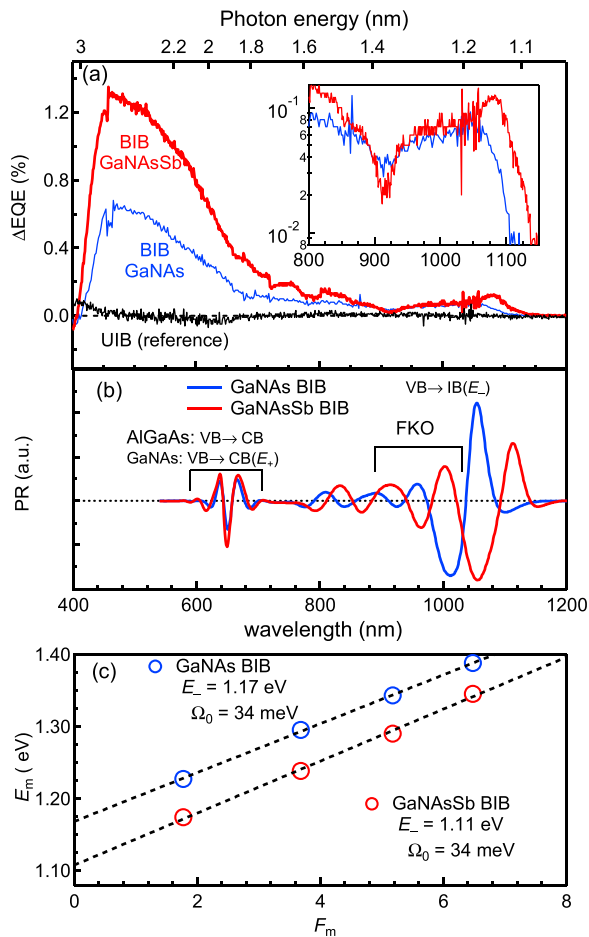
FIG. 23. RT measurements: (a) spectral dependence of \Delta EQE of GaNAs and GaNAsSb BIB structures, respectively. For reference, the \Delta EQE spectrum of a GaNAs UIB structure is also shown in (a). (b) PR spectra of both structures at RT. (c) Linear plot of the E_m of FKO's around IB(E_-) transitions as a function of F_m , which is a reduced parameter for the number ( m ) of the extrema E_m .
