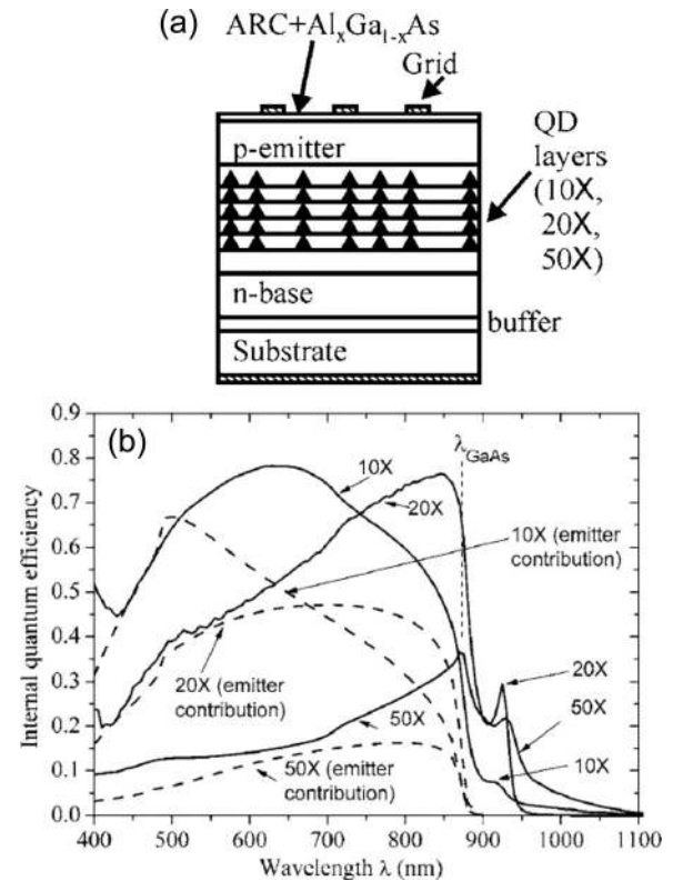
FIG. 29. (a) Simplified internal structure of the IBSCs implemented with QDs and used in these experiments. (b) IQE corresponding to QD-IBSCs with 10, 20, and 50 layers of QD connected lines. The dashed lines correspond to the estimated contribution from the p emitter of the cells. \lambda_{\text{GaAs}} is the GaAs bandgap wavelength and is shown for reference. Reprinted with permission from Martí et al. , Appl. Phys. Lett. 90 , 233510 (2007). Copyright 2007 AIP Publishing LLC.
