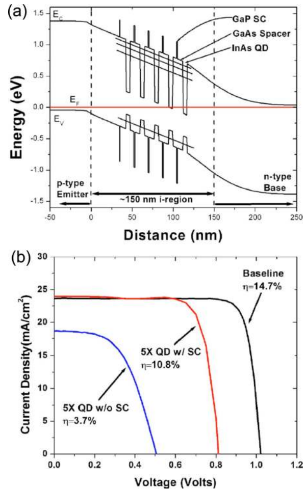
FIG. 32. (a) Simplified energy band diagram illustrating the design of the strain-compensated QDSC. The diagram is generated near the i -region of a p-i-n cell containing InAs QDs with GaP SCL. (b) J - V curves under 1 sun of AM 0 solar spectrum for the p-i-n GaAs control cell and QDSCs both with and without strain-compensation. 5 layers stacked InAs QDs are inserted into the intrinsic layer for all QDSCs. Reprinted with permission from Hubbard et al. , Appl. Phys. Lett. 92 , 123512 (2008). Copyright 2008 AIP Publishing LLC.
