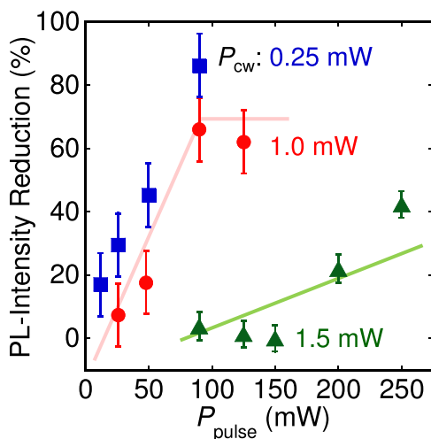
FIG. 65. IR-pulse-excitation-power dependence of the two-color photoexcitation spectroscopy signal as a function of various interband CW-excitation intensity.
