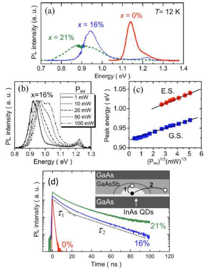
FIG. 34. (a) PL spectra of the GaAs 1-x Sb x covered InAs QDs with different x . (b) Power dependent PL spectra of the InAs QDs covered by GaAs 0.84 Sb 0.16 . (c) The Ground State (G.S.) and the Excited State (E.S.) peak energies as a function of P_{ex}^{1/3} for the InAs QDs covered by GaAs 0.84 Sb 0.16 . (d) TR-PL decay traces for the investigated QD samples with different Sb composition. The inset depicts the sample structure and the underlying recombination processes responsible for the faster one and slower two decay components. Reprinted with permission from Chang et al. , Appl. Phys. Lett. 93, 033107 (2008). Copyright 2008 AIP Publishing LLC.
