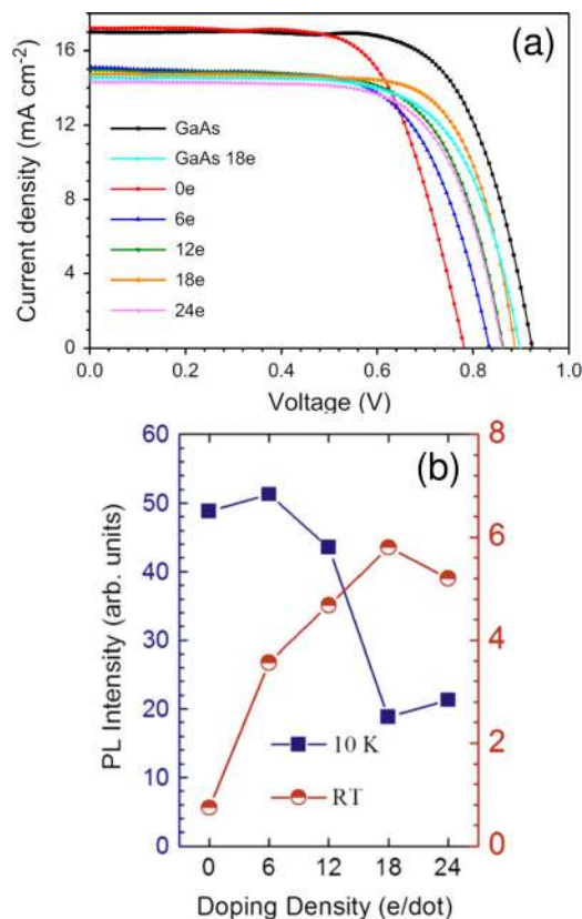
FIG. 43. (a) J - V measurements obtained under 1 sun (AM 1.5G) illumination for Si-doped QDSCs, GaAs cell, and 18e GaAs cell. (b) Integrated PL intensity for Si-doped QDSCs with 0e , 6e , 12e , 18e , and 24e per QD measured at 10 \text{ K} and \text{RT} . Reprinted with permission from Lam et al. , Nano Energy 6, 159 (2014). Copyright 2014 Elsevier B.V.
