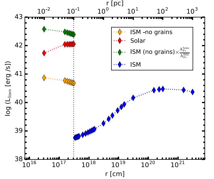
Figure 8. Comparison of Fe II line luminosity for two models of clouds illuminated by the Mrk 509 SED with different abundances of dustless clouds. The ISM composition with grains is used for dusty clouds located further out than R_d , marked by the vertical dotted line. For clouds located closer to the SMBH than R_d we plotted Fe II line luminosity as red diamonds for solar iron abundance and as orange diamonds for the ISM abundance without grains. Green diamonds mark the ISM model without grains multiplied by the Fe abundance ratio of those two models.
