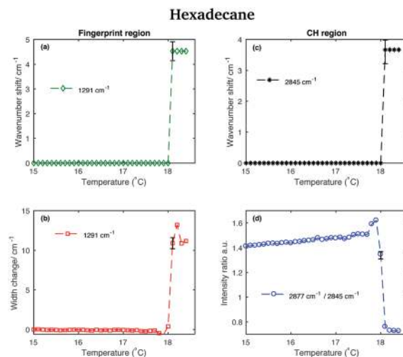
Fig. 12 Changes in the fingerprint and CH stretching region of the Raman spectra of hexadecane as function of temperature. (a) Wavenumber shift of the twisting band (at 1291 \text{ cm}^{-1} in the spectrum of solid hexadecane) as function of temperature. (b) Width change of the twisting band as function of temperature. (c) Wavenumber shift of the \text{CH}_2 symmetric stretching band (at 2845 \text{ cm}^{-1} in the spectrum of solid hexadecane) as function of temperature. (d) Intensity ratio of the \text{CH}_2 asymmetric and symmetric stretching bands (at 2877 \text{ cm}^{-1} and at 2845 \text{ cm}^{-1} in the spectrum of solid hexadecane, respectively).
