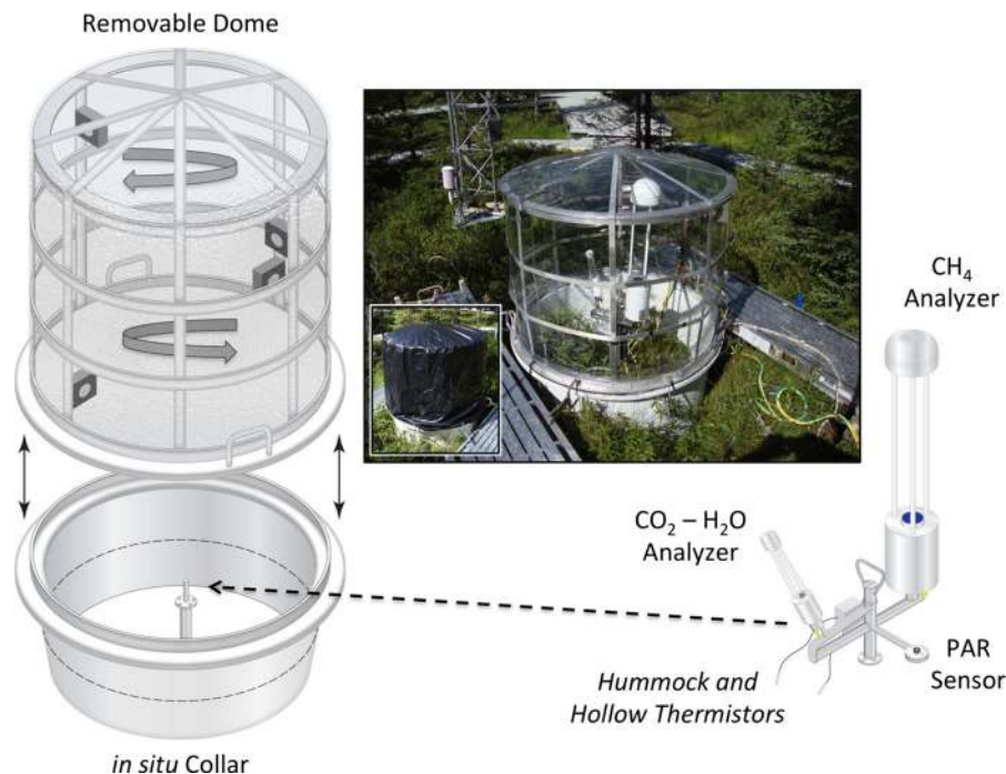
Fig. 1 Diagrams and photographs of the complete CH 4 –CO 2 –H 2 O measurement system installed for observations in the S1-Bog. A permanent in situ collar and instrument stand remain in the peatland. The instrument package and transparent dome are assembled in and over the collar, respectively, for each short term measurement. The photograph shows the transparent
