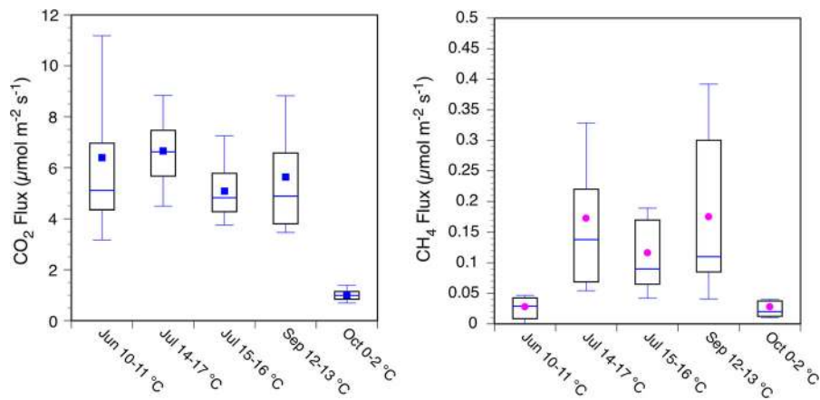
Fig. 5 Spatial variation statistics in “dark condition” CO 2 flux ( left graph ) and CH 4 flux ( right graph ) for multiple locations across a 2.6 ha experimental area at the south end of the S1-Bog. The box-and-whisker plots capture 10, 25, 75 and 90th percentiles of the spatial data along with the overall median (50th percentile) and the symbol is the mean of the spatial data
