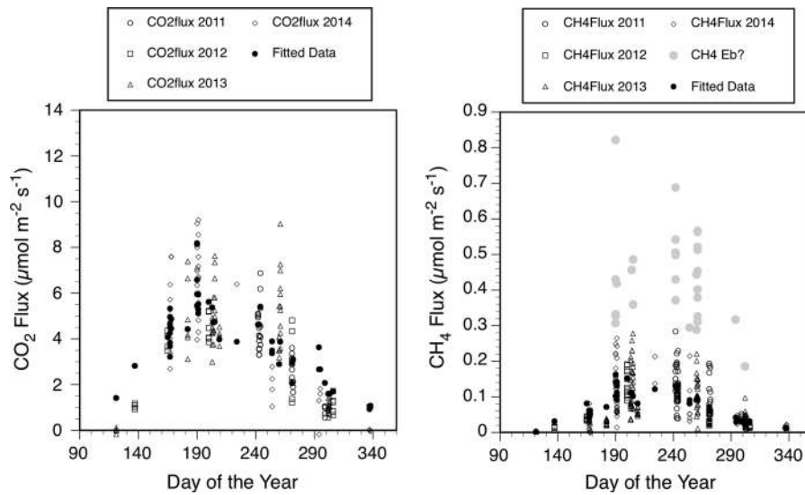
Fig. 3 Periodic observations of dark-daytime CO 2 (left graph) and CH 4 (right graph) efflux measured throughout the active seasonal cycle for the S1-Bog. Data represent the combined observations from measurements collected from variable plot locations on the S1-Bog in 2011, 2012, 2013 and 2014. Fitted
