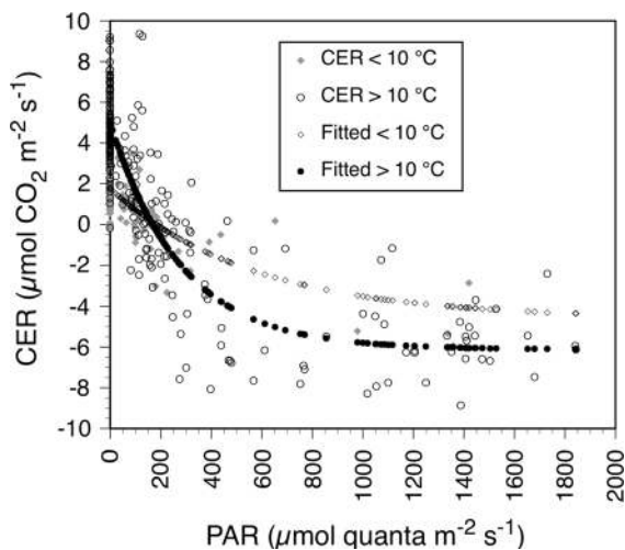
Fig. 4 Net community CO 2 exchange for the collared area under ambient light conditions. Negative values represent CO 2 uptake from the atmosphere to the bog. Gray solid diamonds and open circles represent data collected at surface peat temperatures below or above 10 °C. The open diamonds and black circles are the fitted data for the data obtained below and above the 10 °C surface soil temperatures
