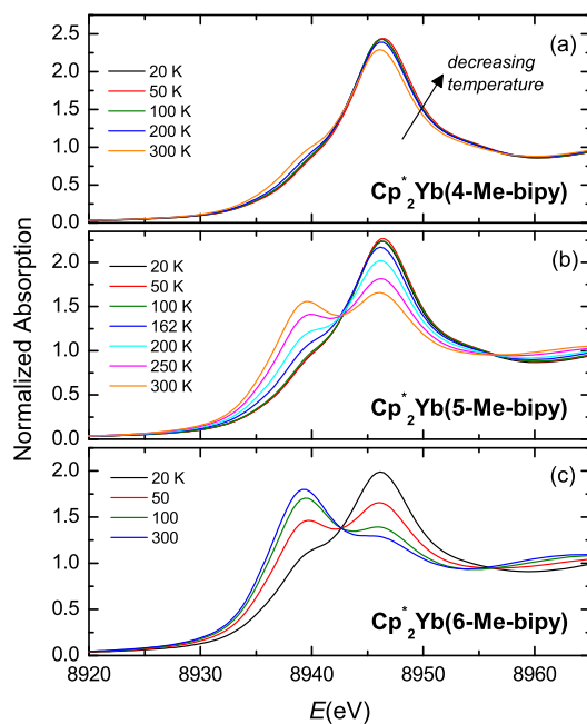
Figure 3: Yb L_{III} -edge XANES data for \text{Cp}_2^*\text{Yb}(\text{x-Me-bipy}) complexes at various temperatures.
