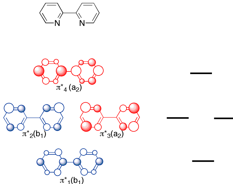
Figure 9: The \pi^* orbitals on the bipy ligand in C_{2v} symmetry. Circle size is proportional to the electron density, and open circles are out of phase with closed circles. Adapted from Ref. 40
