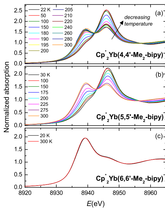
Figure 4: Yb L_{III} -edge XANES data for \text{Cp}_2^*\text{Yb}(\text{x,x}'\text{-Me}_2\text{-bipy}) complexes at various temperatures.
