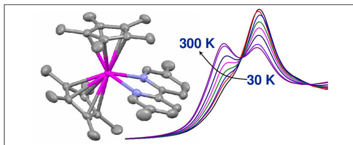
Graphic displays the Yb L_{\text{III}} edge XANES of \text{Cp}_2^+\text{Yb}(5,5'\text{-Me}_2\text{-bipy}) as a function of temperature, demonstrating the change in Yb oxidation state and the intermediate valence tautomerism.
