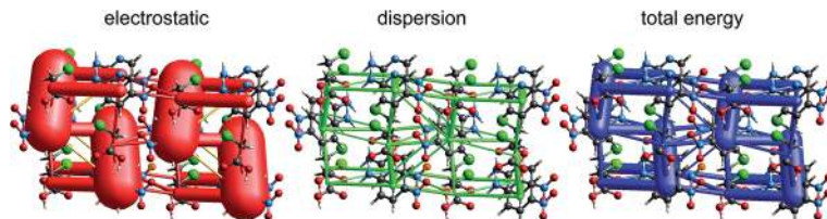
Fig. 13 2-Amino-5-pyridine:chloroacetic acid co-crystal (TETXUL01): energy frameworks for separate electrostatic (red) and dispersion (green) contributions to the total nearest neighbour pairwise interaction energies (blue). See Fig. 10 for details.
