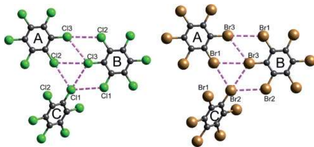
Fig. 16 Closest \text{Cl} \cdots \text{Cl} and \text{Br} \cdots \text{Br} contacts (magenta dashed lines) between adjacent molecules in hexachlorobenzene (HCLBNZ12) and hexabromobenzene (HBRBEN02). The atom labelling is the same as that in the original CIF files. See Table 1 for interaction energies between molecules A, B and C, as well as those involved in the stacking motif.
