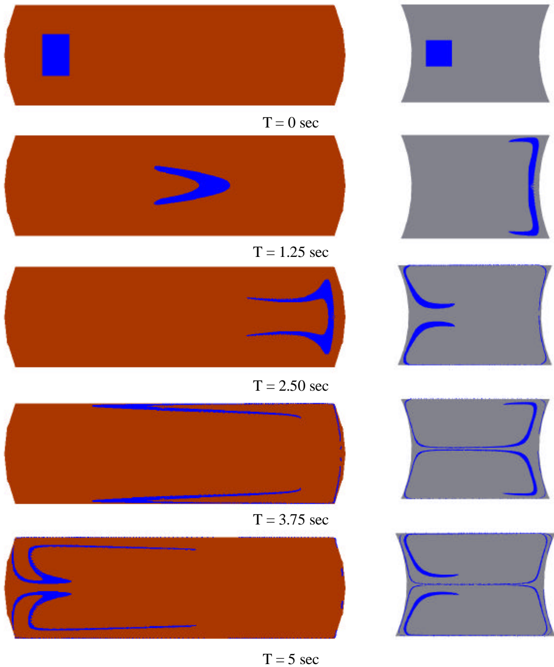
Figure 9. Internal circulations by particle tracing in aqueous and organic slugs respectively. ( V_{av} = 5.64 mm/s, D = 0.75 mm)
