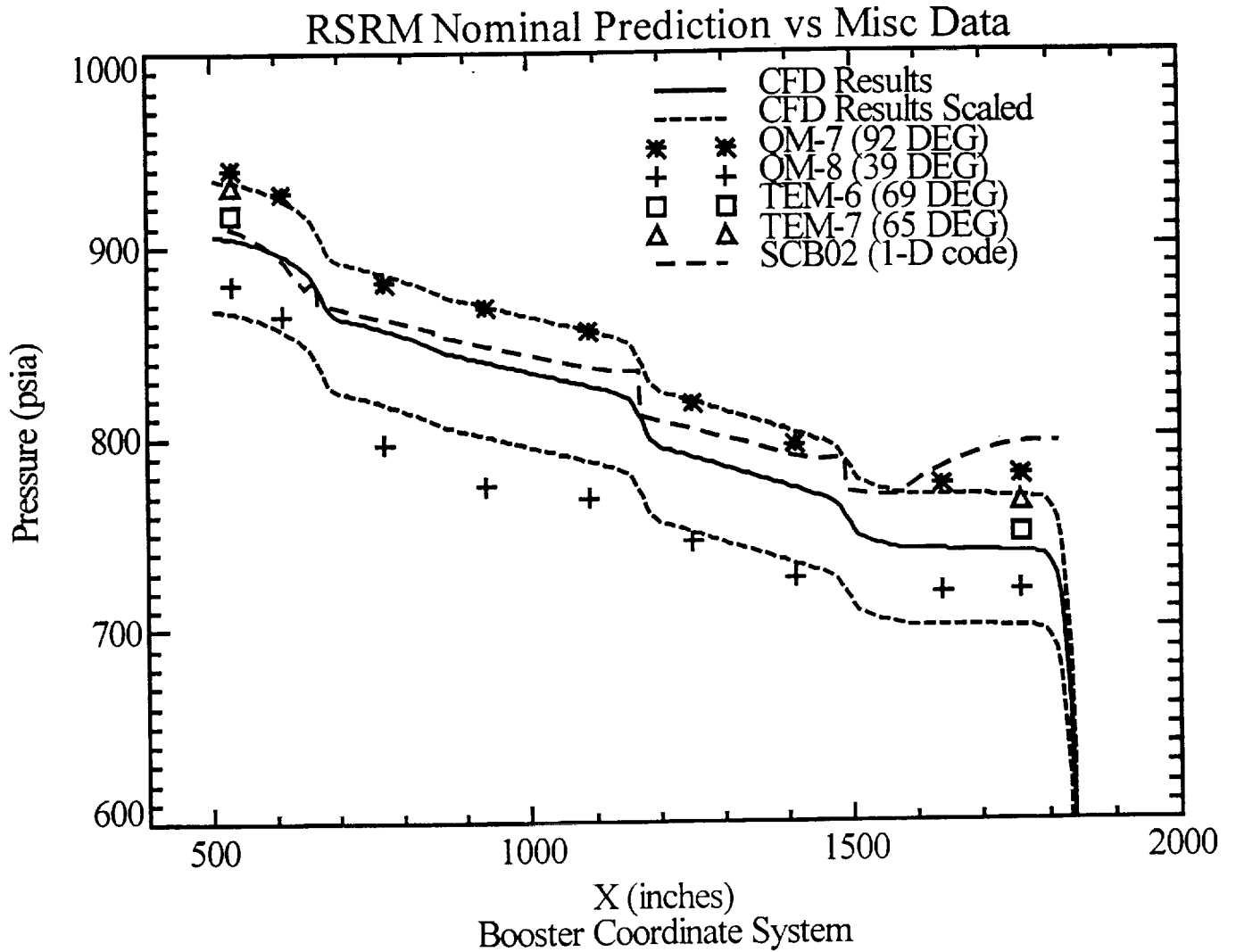
Figure 6 RSRM Baseline CFD Model Calibration (TVR=10,000)
