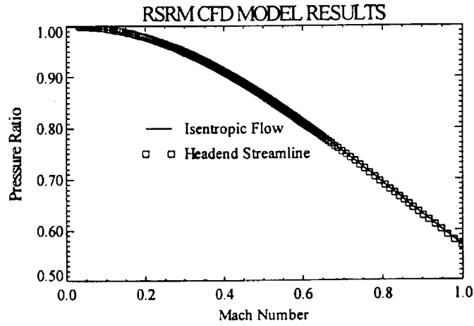
Figure 11 Pressure Ratio Versus Mach Number
