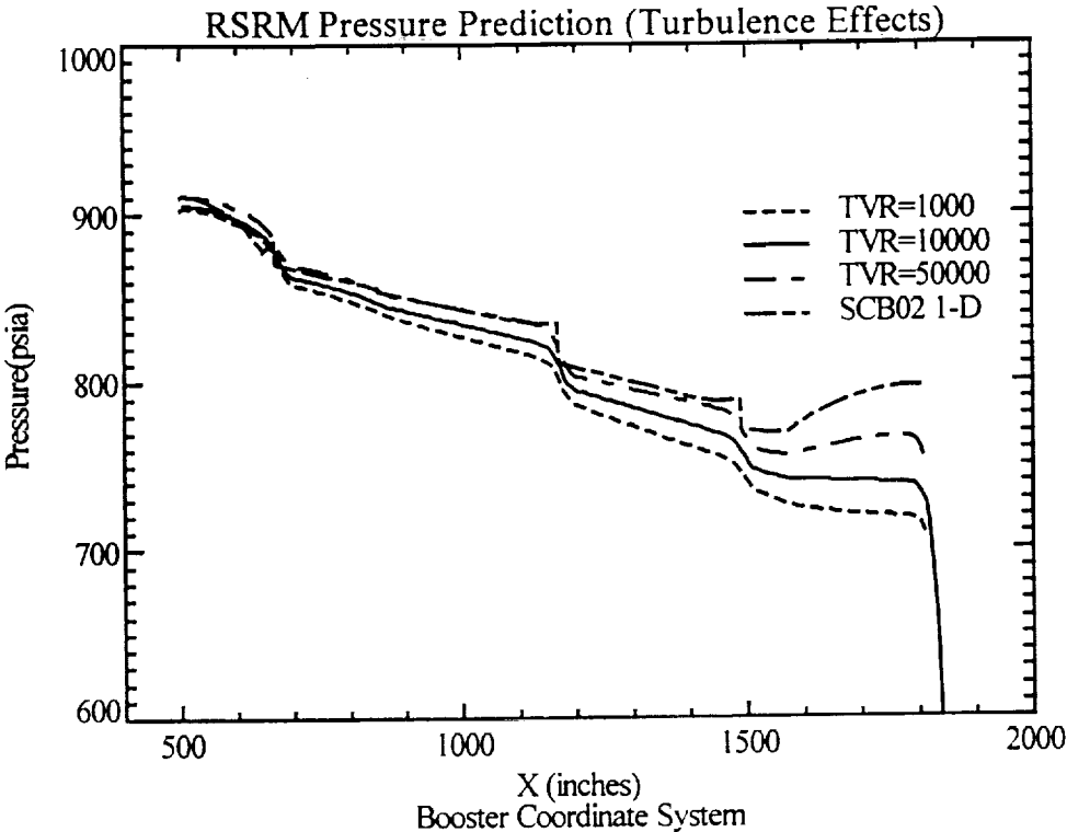
Figure 4 RSRM Pressure Prediction with Turbulence Effects
