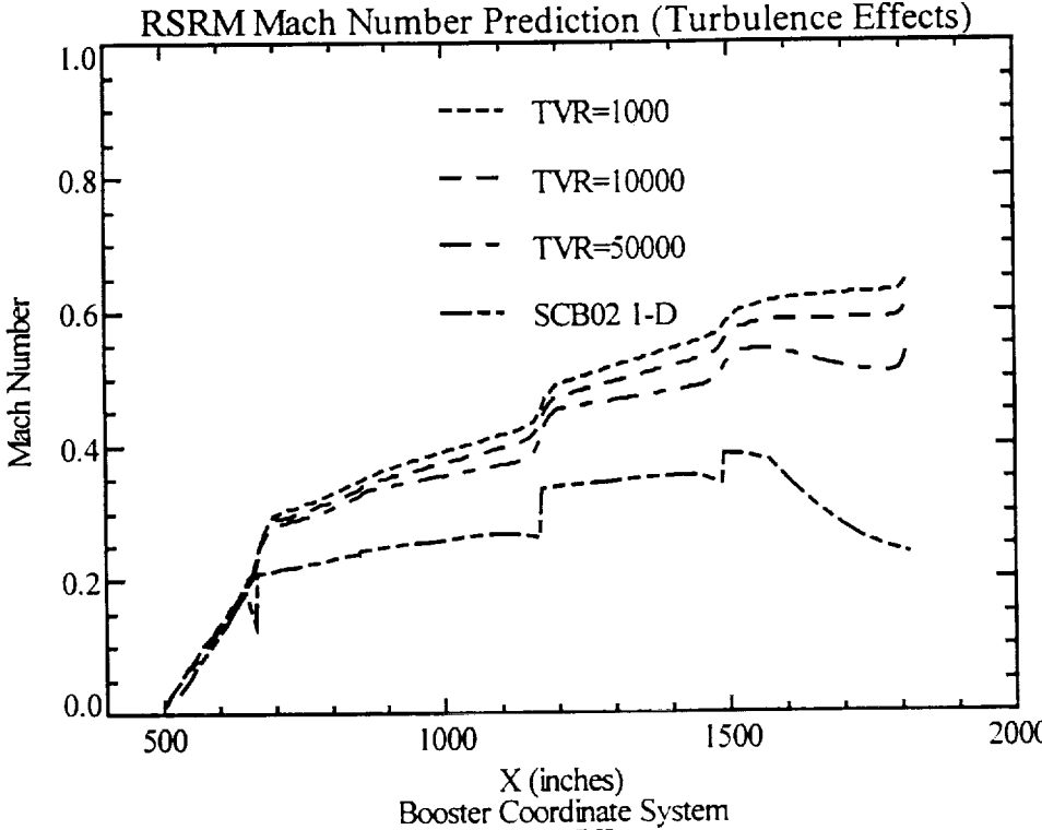
Figure 5 RSRM Mach Number with Turbulence Effects
