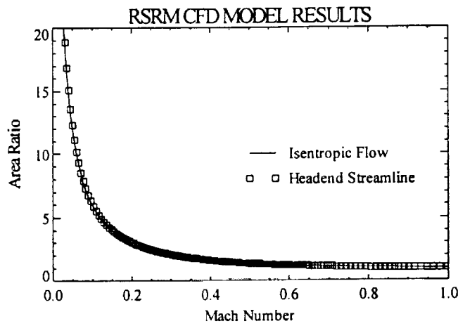
Figure 12 Area Ratio Versus Mach Number
