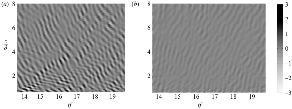
FIGURE 5. (a) Upward and (b) downward propagating wave components of \partial w'/\partial z in a frame moving with U_\infty , for Ri_* = 1000 and Re_* = 960 .
