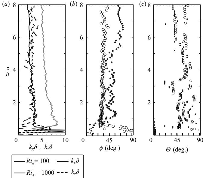
FIGURE 9. Characteristics of waves with the largest amplitude of \partial w'/\partial z for Re_* = 960 . Here \phi is the azimuthal angle and \Theta is the polar angle. (b,c) ●, Ri_* = 100 ; ○, 1000.
