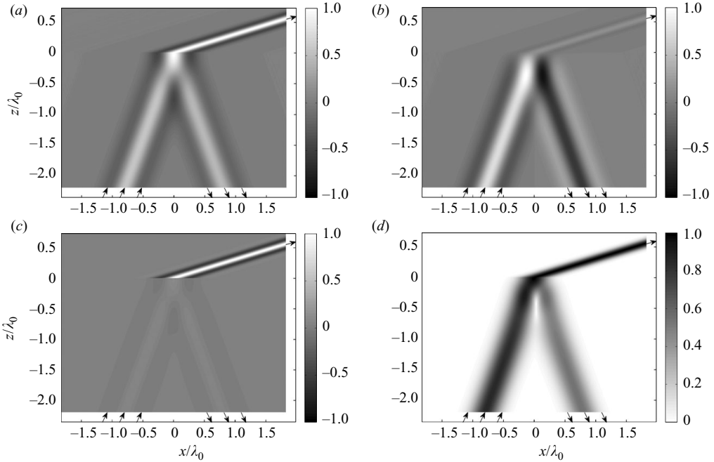
FIGURE 2. Wave beam transmission across a sharp density-gradient interface. (a) u . (b) w . (c) \Delta N^2 . (d) \bar{e} . The frequency ratios are \omega/N_1=0.94 and N_2/N_1=3.2 . Arrows specify the direction of energy propagation. The maximum value in each figure is scaled to unity, and the spatial scales have been non-dimensionalized by the dominant wavelength, \lambda_0 , in \psi_I(k) . The dominant wavelength is defined as \lambda_0 = 2\pi/k_0 , where \psi_I(k) is maximum at k = k_0 .
