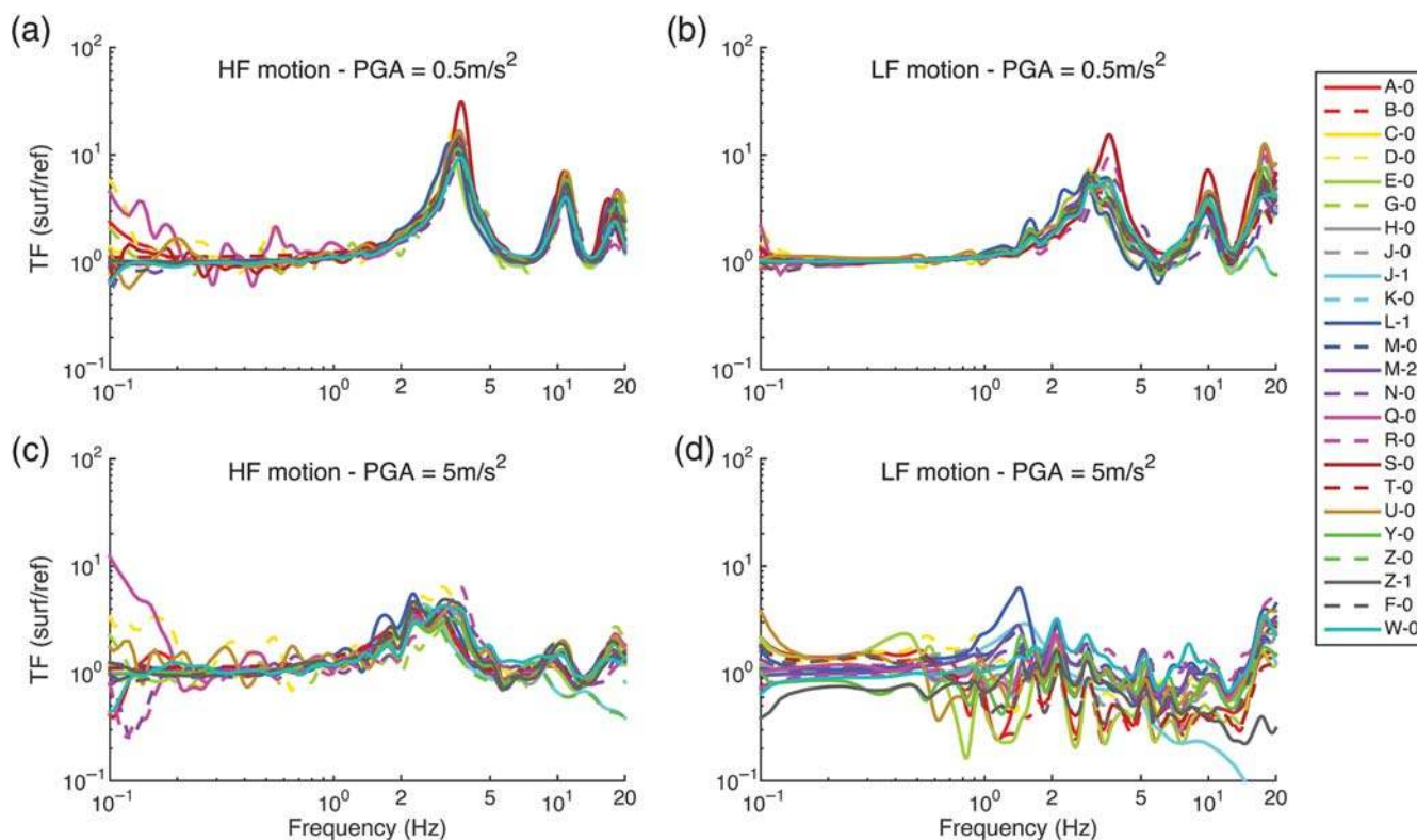
Figure 9. Comparison of the surface to reference Fourier spectra ratio, for the nonlinear (NL) computations using the HF input motion (a) scaled to 0.5 m/s 2 and (c) scaled at 5 m/s 2 , and using the LF input motion (b) scaled to 0.5 m/s 2 and (d) scaled at 5 m/s 2 .
