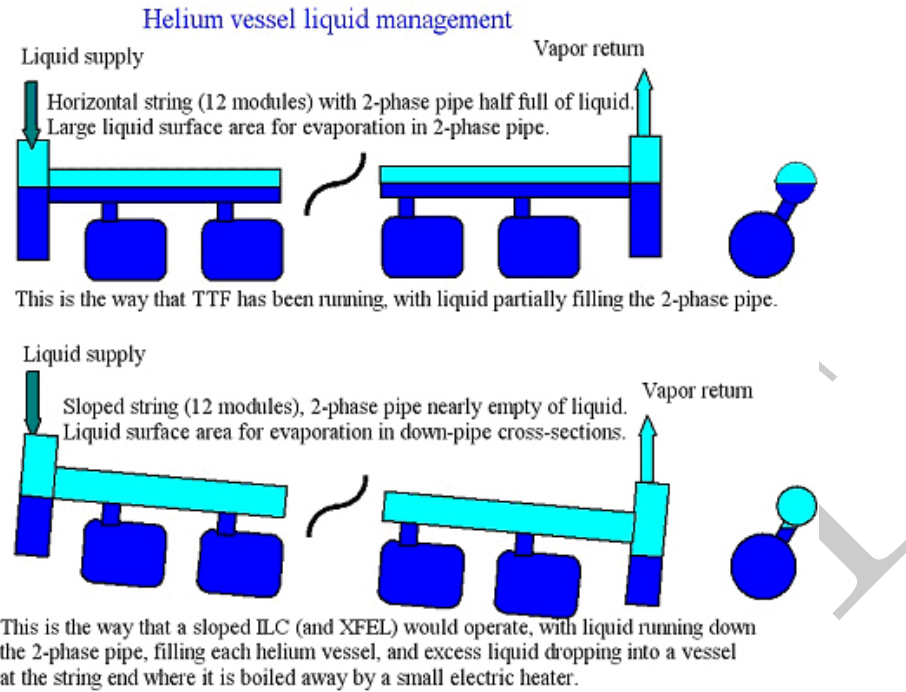
FIGURE 3.8-4. Two-Phase Helium Flow for Level and for Sloped Systems
