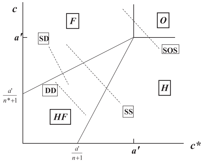
Figure 1. Illustrative Equilibrium Configurations for Given n and n^*
