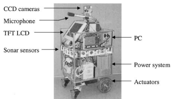
Figure 1. The IPR hardware.
