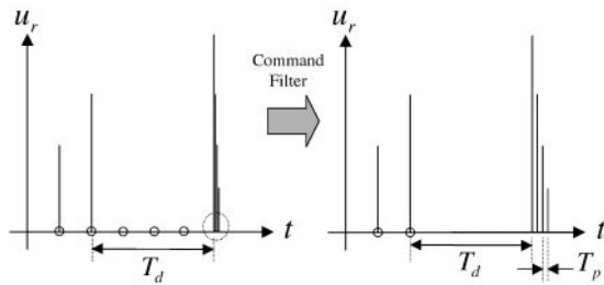
Figure 8. Function of the modified command filter .
