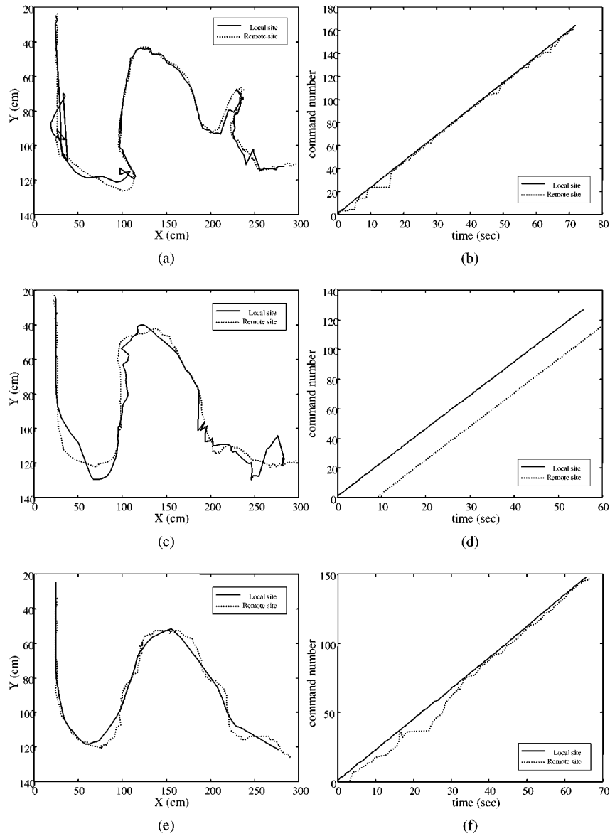
Figure 16. Experimental results. (a) Path error (internet control architecture-I). (b) Time difference (internet control architecture-I). (c) Path error (internet control architecture-II). (d) Time difference (internet control architecture-II). (e) Path error (internet control architecture-III). (f) Time difference (internet control architecture-III).
