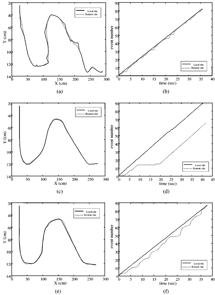
Figure 12. Simulation results. (a) Path error (internet control architecture-I). (b) Time difference (internet control architecture-I). (c) Path error (internet control architecture-II). (d) Time difference (internet control architecture-II). (e) Path error (internet control architecture-III). (f) Time difference (internet control architecture-III).
