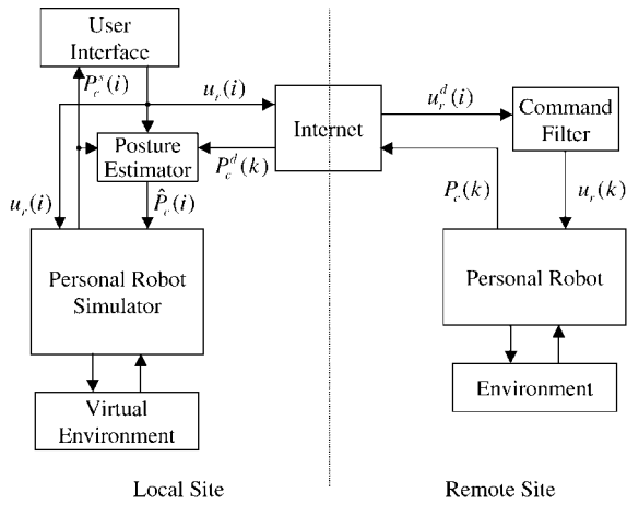
Figure 6. Internet control architecture-II (Step 2).
