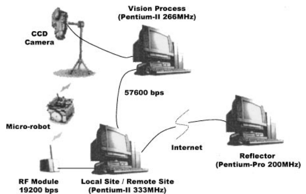
Figure 14. Overview of the experiment settings.
