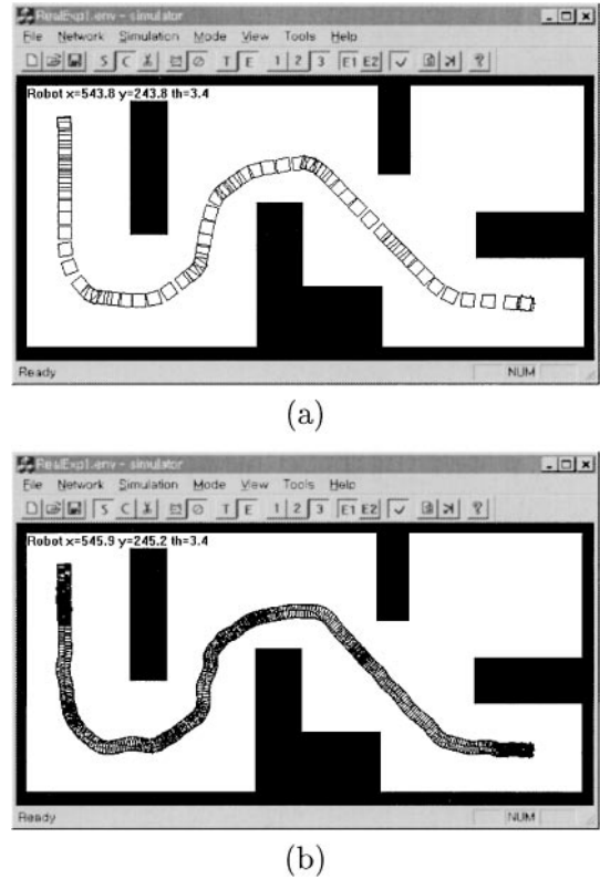
Figure 11. Simulation results by the internet control architecture-III. (a) Virtual robot path at the local site. (b) Real robot path at the remote site.
