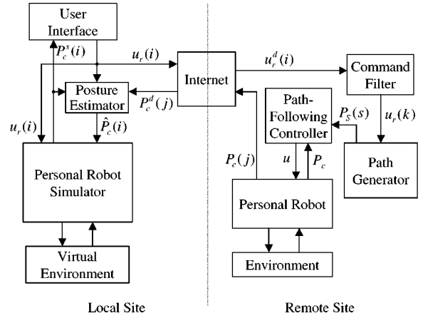
Figure 9. Internet control architecture-III (Step 3).
