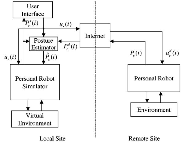
Figure 5. Internet control architecture-I (Step 1).
