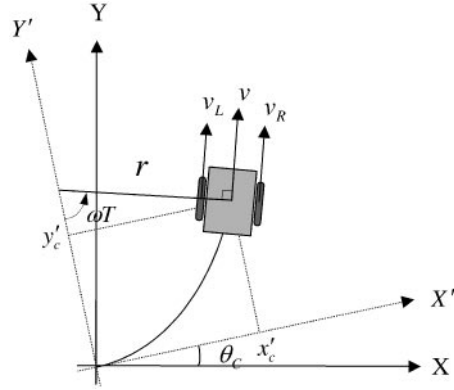
Figure 2. Trajectory of a mobile robot.
