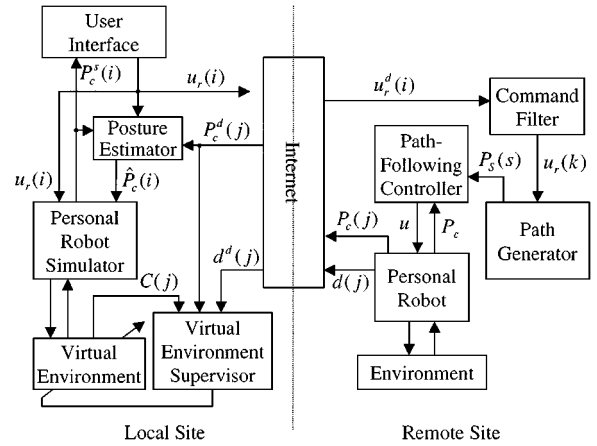
Figure 10. Extended internet control architecture.
