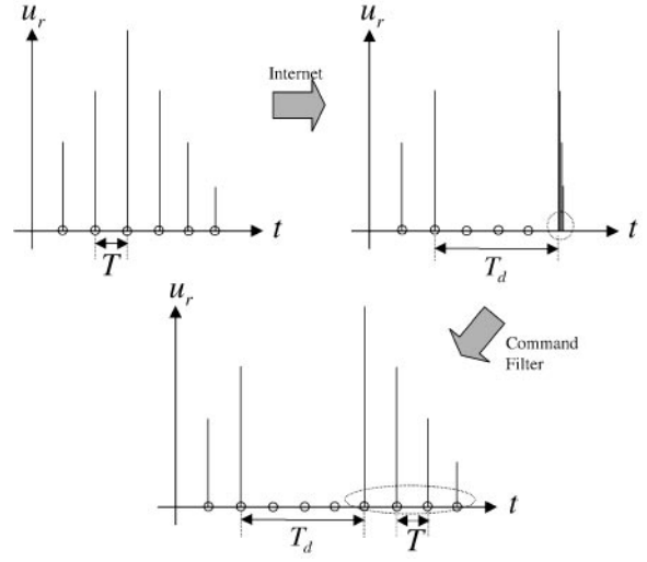
Figure 7. Function of command filter.
