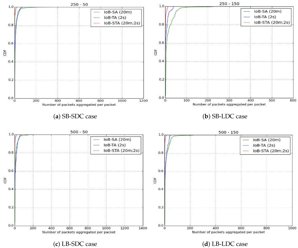
Figure 43. Average number of aggregated packets per packet for IoB-SA.
