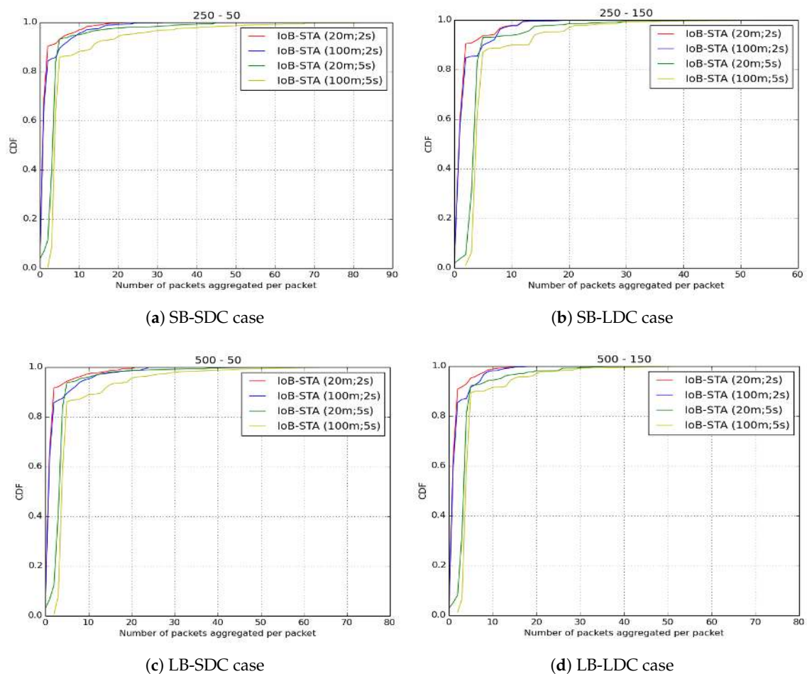
Figure 38. Average number of aggregated packets per packet for IoB-STA.
