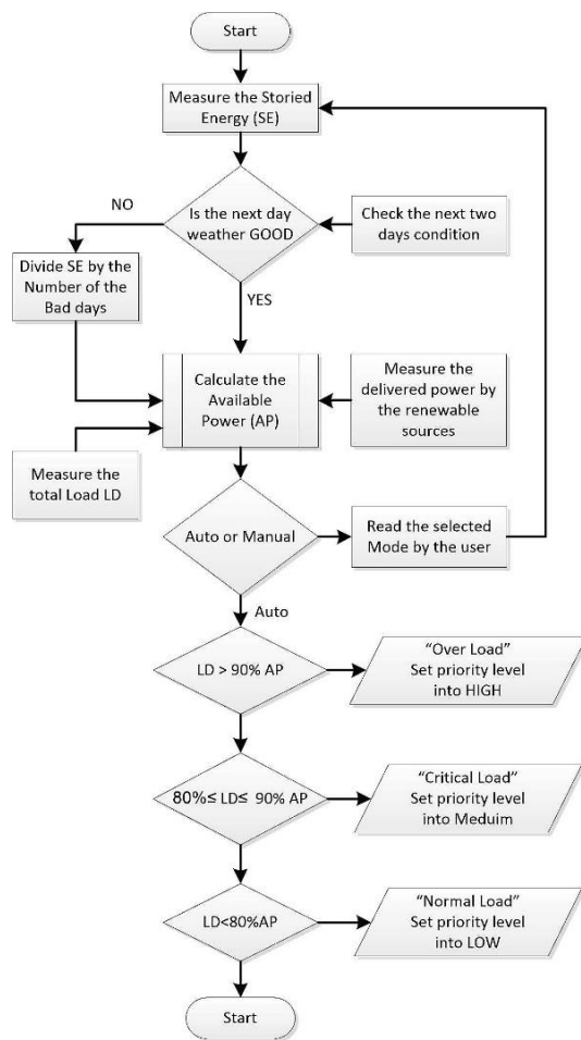
Figure 16. Decision making flowchart.
