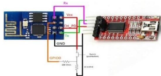
(a) Programming Adapter schematic.
