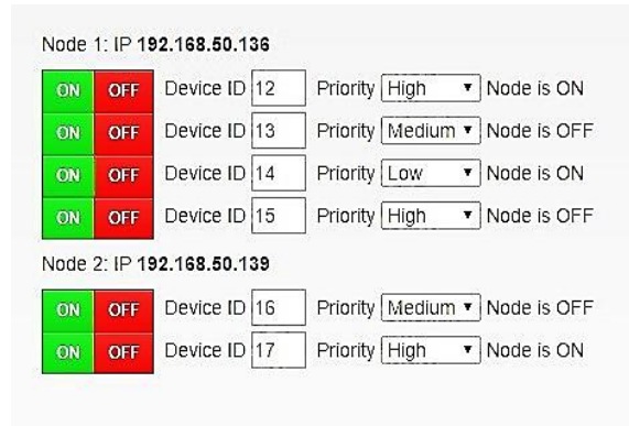
Figure 5. Device Manager.
