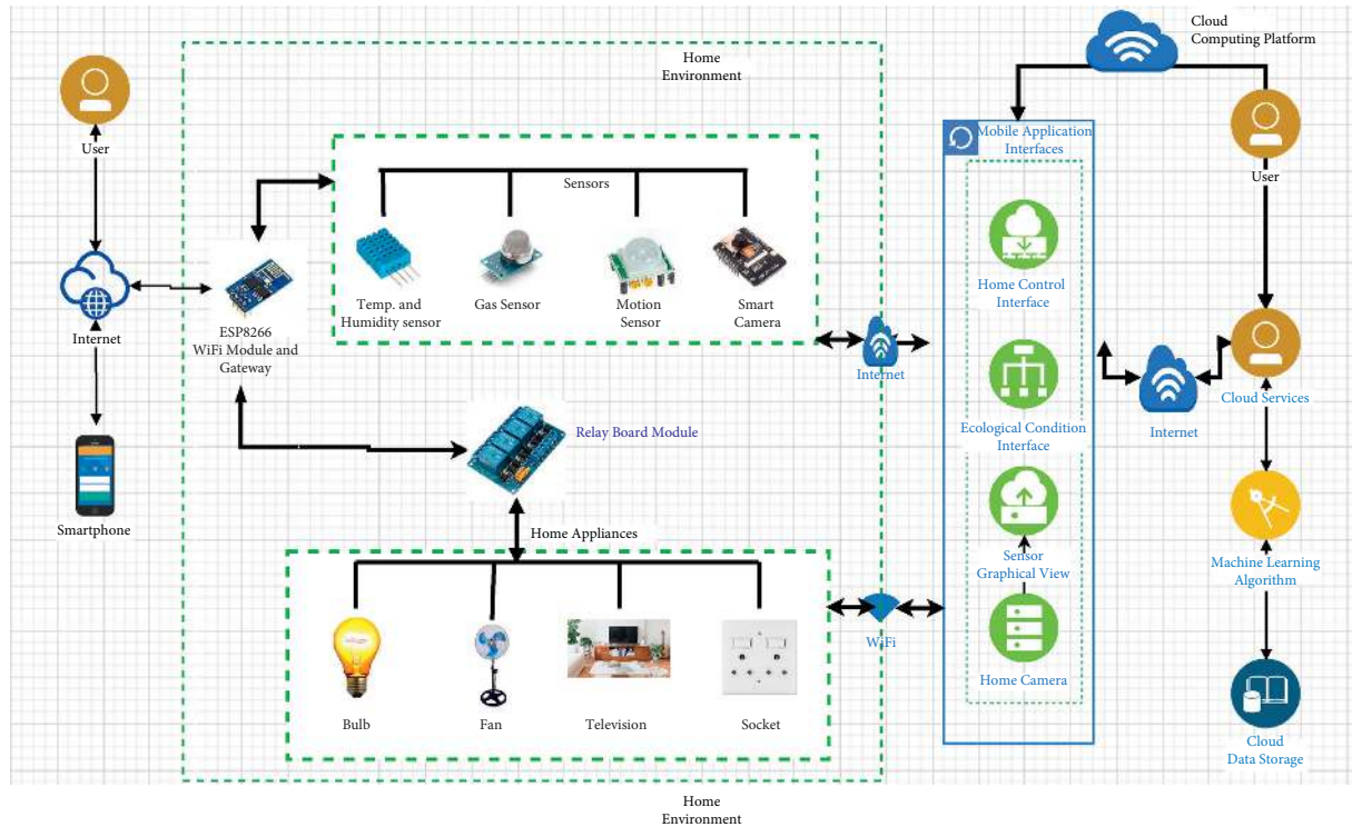
FIGURE 1: The iHOCS architecture.
