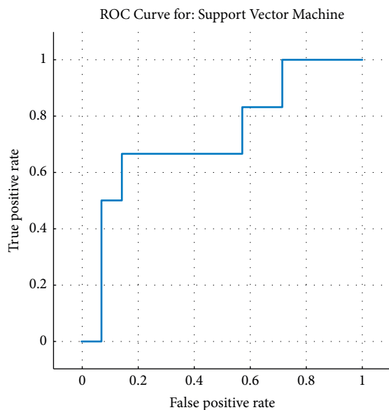
FIGURE 5: SVM ROC curve.
