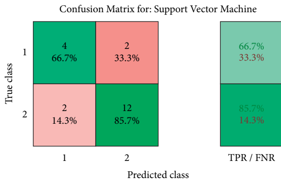
FIGURE 4: SVM confusion matrix.
