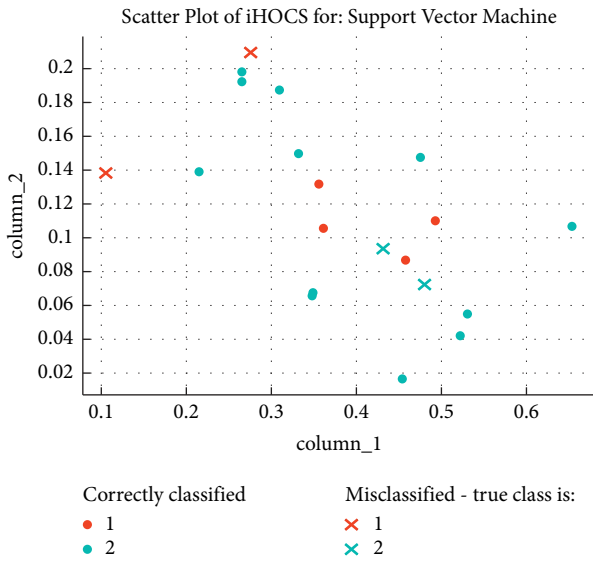
FIGURE 3: SVM scatter plot diagram.
