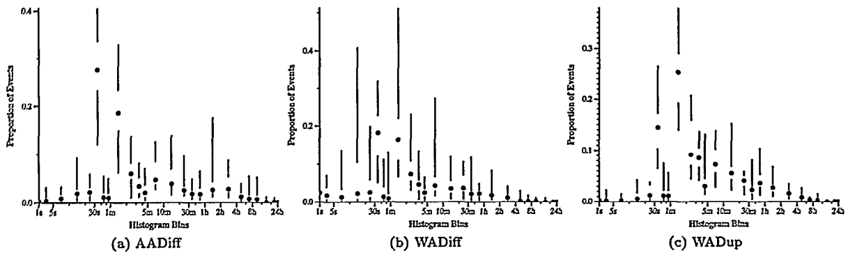
Figure 8: Histogram distribution of update inter-arrival time distances for Prefix+AS instability measured at the Mae-East exchange point during August 1996.
