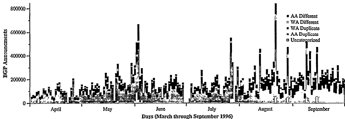
Figure 2: Breakdown of Mae-East routing updates from April through September 1996.
