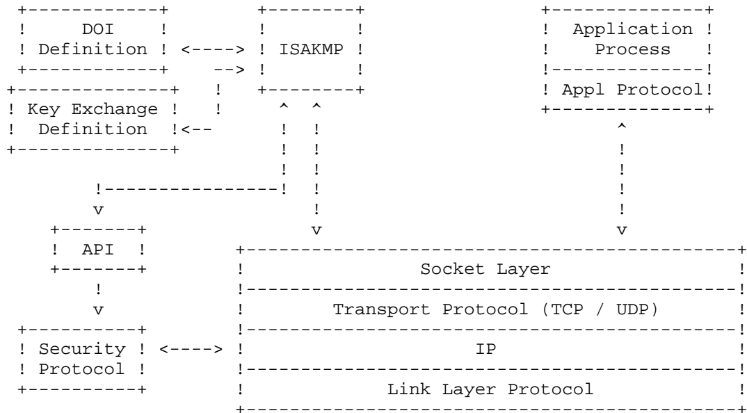
Figure 1: ISAKMP Relationships
