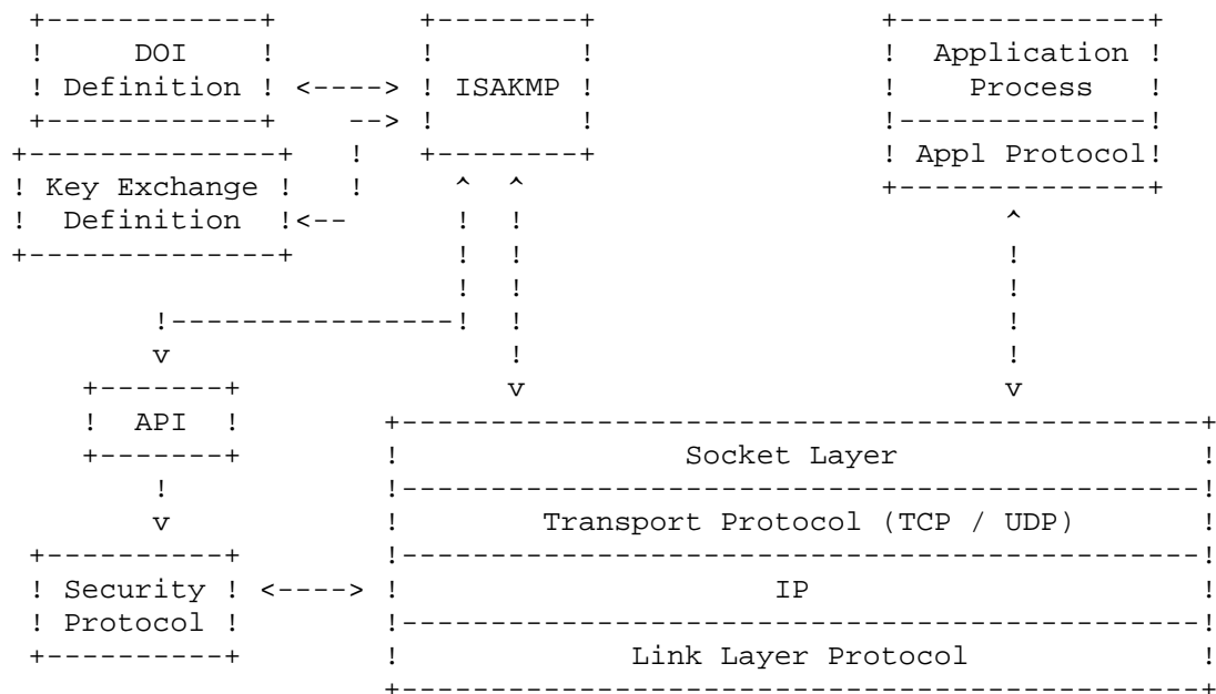
Figure 1: ISAKMP Relationships
