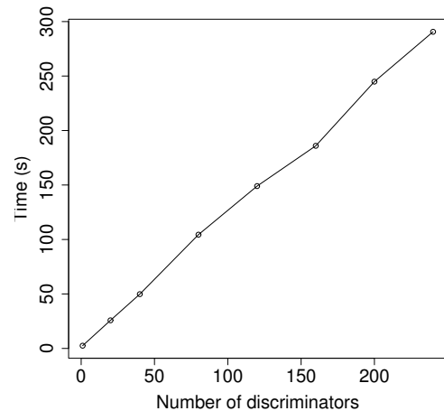
Figure 5: Time taken to build a model on a training set (24863 flows) and test it against the test set (23801 flows) in relation to the number of discriminators in consideration.
