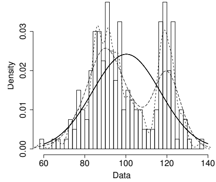
Figure 3: Different estimators of the density that generated the data. The black line represents the Gaussian density whose parameters were estimated from the data, the two dashed lines represent the kernel estimated density with two different values of the bandwidth.
