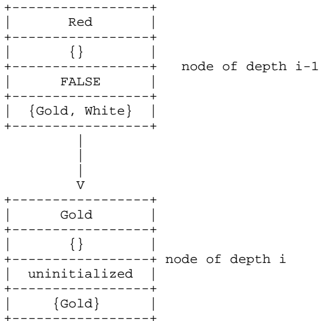
Figure 4. Processing an exact match
