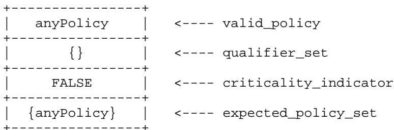
Figure 3. Initial value of the valid_policy_tree state variable
