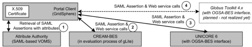
Figure 6. SAML-based Attribute Authority (here VOMS) as crucial authorization element releasing SAML assertions with attribute information used in cross-Grid authorization. SAML assertions can transported with Web service invocations for later authorization checks within the middlewares.
