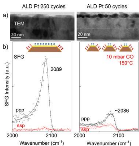
Figure 1. (a) Cross-sectional TEM micrographs of 250 cycle and 50 cycle Pt films. The 250 cycle film consists of large uniform and planar islands (~10 nm in thickness), whereas the 50 cycle film is made up of individual Pt particles (size of about 8 nm). (b) SFG spectra in two different polarization combinations (ppp and ssp) of adsorbed CO (10 mbar at 150 °C); the surface morphology of islands/particles (see models) can be assessed by comparing the ppp to ssp intensity (ppp (ssp) has a higher intensity if the C=O bond is parallel (tilted) to the macroscopic surface normal).
