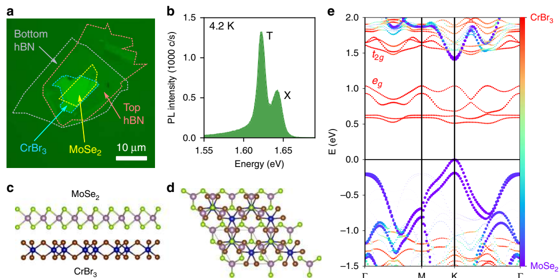
Fig. 1 MoSe 2 /CrBr 3 van der Waals heterostructures. a Microscope image of the sample in this work showing multi-layered CrBr 3 , monolayer MoSe 2 , and hBN encapsulation layers. b Photoluminescence spectrum from the sample under continuous-wave laser excitation at 1.946 eV and a sample temperature of 4.2 K. Neutral exciton (X) and trion (T) peaks are visible. c, d Schematics of a MoSe 2 /CrBr 3 heterobilayer structure used in the density functional theory calculations, viewed from the side ( c ) and top ( d ), where the supercell is highlighted. Here, the experimental lattice constant of monolayer MoSe 2 is applied to both layers, in order to simplify the calculations, along with setting the relative crystallographic twist angle to zero between the layers (see Supplementary Note 1). Crystal images were produced using VESTA software 33 . e The DFT calculated electronic band structure of the MoSe 2 /CrBr 3 heterobilayer, projected on the host material. The global valence band maximum is localized in MoSe 2 at E = 0 . The green band color indicates hybridization between the two materials. The e_g -orbitals have spin polarization opposite to the t_{2g} -orbitals.
