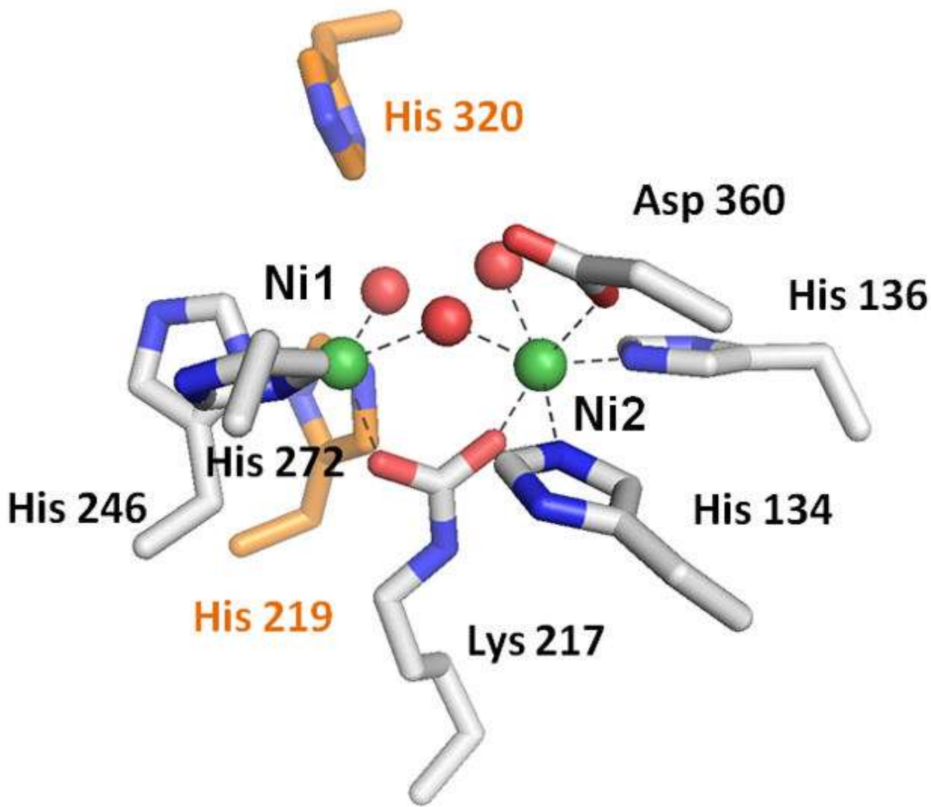
Fig. 2. The urease active site. The active site of urease contains two nickel atoms (green) bridged by a carboxylated lysine and a hydroxyl group. Ni1 is also coordinated by two histidine residues and a solvent molecule, while Ni2 is coordinated by two histidines, an aspartic acid residue, and a water molecule. Waters are red, metal-binding side chains are shown with white carbon atoms, and two nearby histidine residues that function in catalysis are shown with orange carbon atoms.
