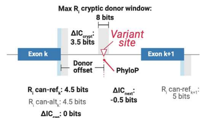
Figure 3. Features are extracted and generated for the donor and acceptor sites and leveraged for random forest learning, whose predictions are calibrated by logistic regression to provide the final SQUIRLS predictions. A) SQUIRLS calculates 7 features to evaluate variant impact on the donor site. The individual information content ( R_i ) of the reference and alternate canonical splice site and of the donor site in the following exon (Exon k+1 ) are calculated and used to determine the difference in information content between the reference and alternate canonical splice site ( \Delta IC_{can} ), the difference between the best candidate cryptic splice site and the alternate sequence of the canonical splice site ( \Delta IC_{crypt} ) and the difference between the donor site at exon k and k+1 ( \Delta IC_{next} ). See Table 1 for information about other features. B) In this example, a variant in intron k creates a cryptic splice site with 8 bits, which is greater than in the
