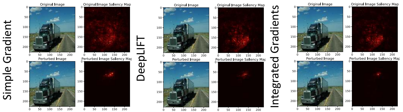
Figure 5: Targeted attack against feature importance map. Image is correctly classified as “trailer truck”. For all methods, the devised perturbation with \epsilon = 8 was able to semantically meaningfully change the focus of saliency map to the “cloud” above the truck. (The cloud area was captured using SLIC (Achanta et al. 2012) superpixel segmentation.) ( top ) as well as rank order correlation ( bottom ).
