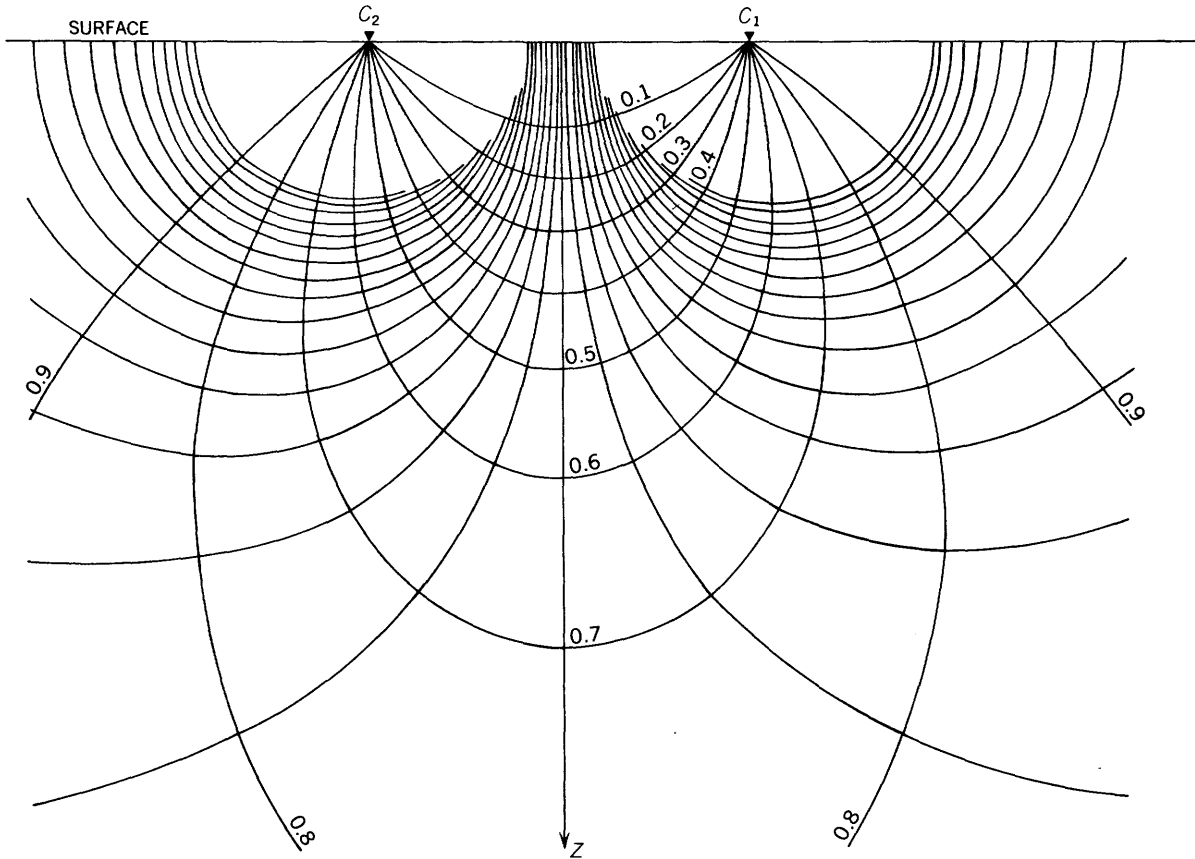
FIGURE 4.—Potential and current distribution in a vertical plane along the line of electrodes. Current lines of flow represent the surfaces of spindles each of which carries one-tenth of the total current. The potential drop between successive equipotential lines is constant. Adapted from Stefanescu (1929).
