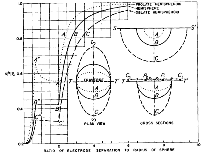
FIGURE 153.—Theoretical vertical resistivity profiles over hemispheroidal sinks. Profiles taken along traverse TT' with center of configuration at center of hemispheroids. \rho''/\rho' = 1/5 . Adapted from Cook and Van Nostrand (1954).
