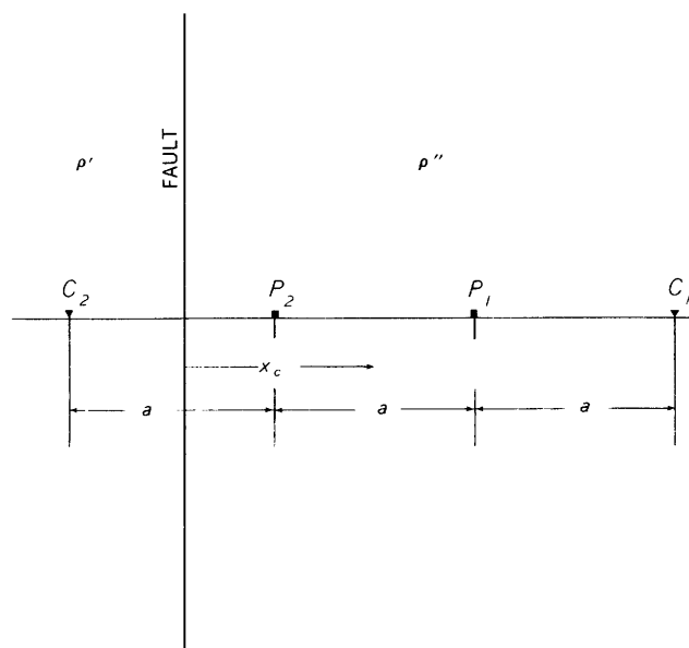
FIGURE 17.—Plan view of the Wenner configuration oriented perpendicular to a vertical fault.
