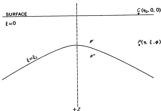
FIGURE 169.—Cross section of a buried dome structure.
