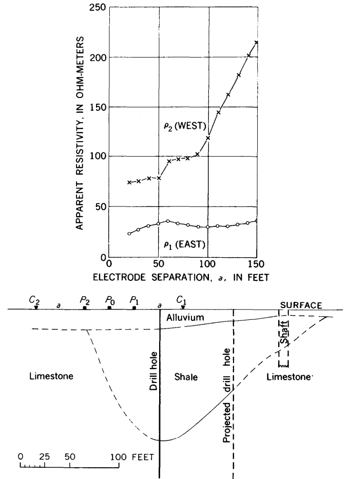
FIGURE 60.—Vertical resistivity profile for station near left edge of shale sink, Lee configuration. Tri-State mining district, Cherokee County, Kans. (Resistivity data and interpretations by K. L. Cook (1951-54); drill-hole data from Brichta and Ryan (1958).)
