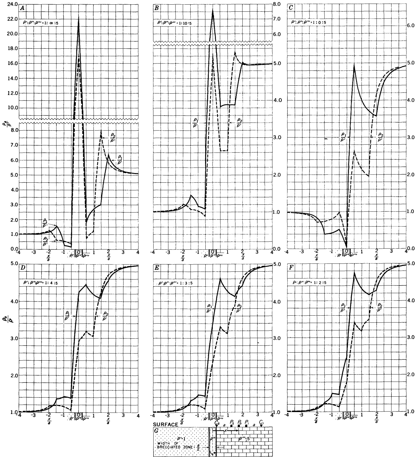
FIGURE 70.—Horizontal resistivity profiles across brecciated zone of different resistivities, Lee configuration (offset plotting). For all diagrams \rho''/\rho''' = 1:5 and width is a/2 .
