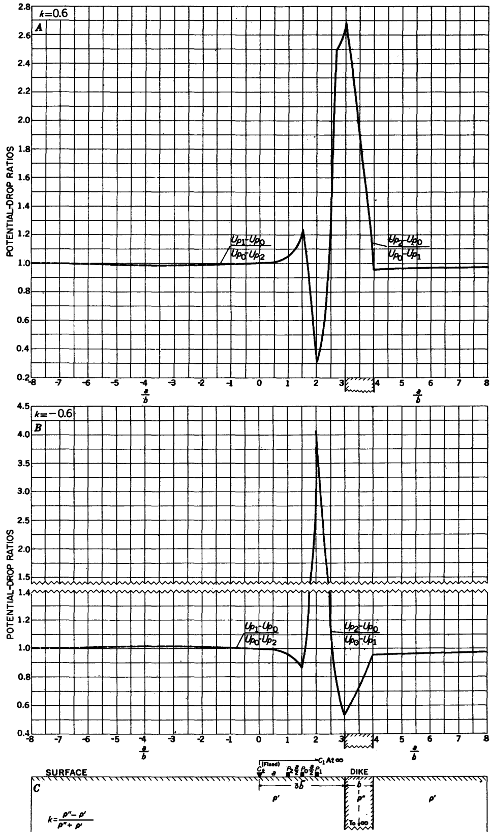
FIGURE 109.—Profiles with expanding-electrode system of potential-drop-ratio method across a vertical dike of width b , with current electrode C_1 at a fixed distance 3b from the dike. Data are normalized. Reflection factors are (A) k=+0.6 ; (B) k=-0.6 .
