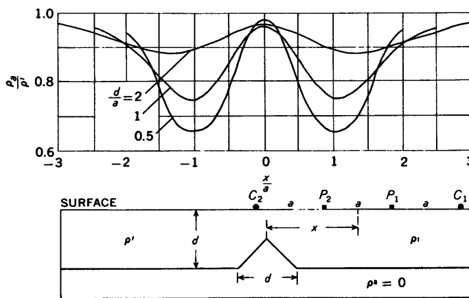
FIGURE 196.—Horizontal resistivity profiles across buried perfectly conducting symmetrical anticlines of different sizes and depths of burial, Wenner configuration (two-dimensional approximation); a= unity. Adapted from Kiyono (1950c) by permission of Kyōtō University.
