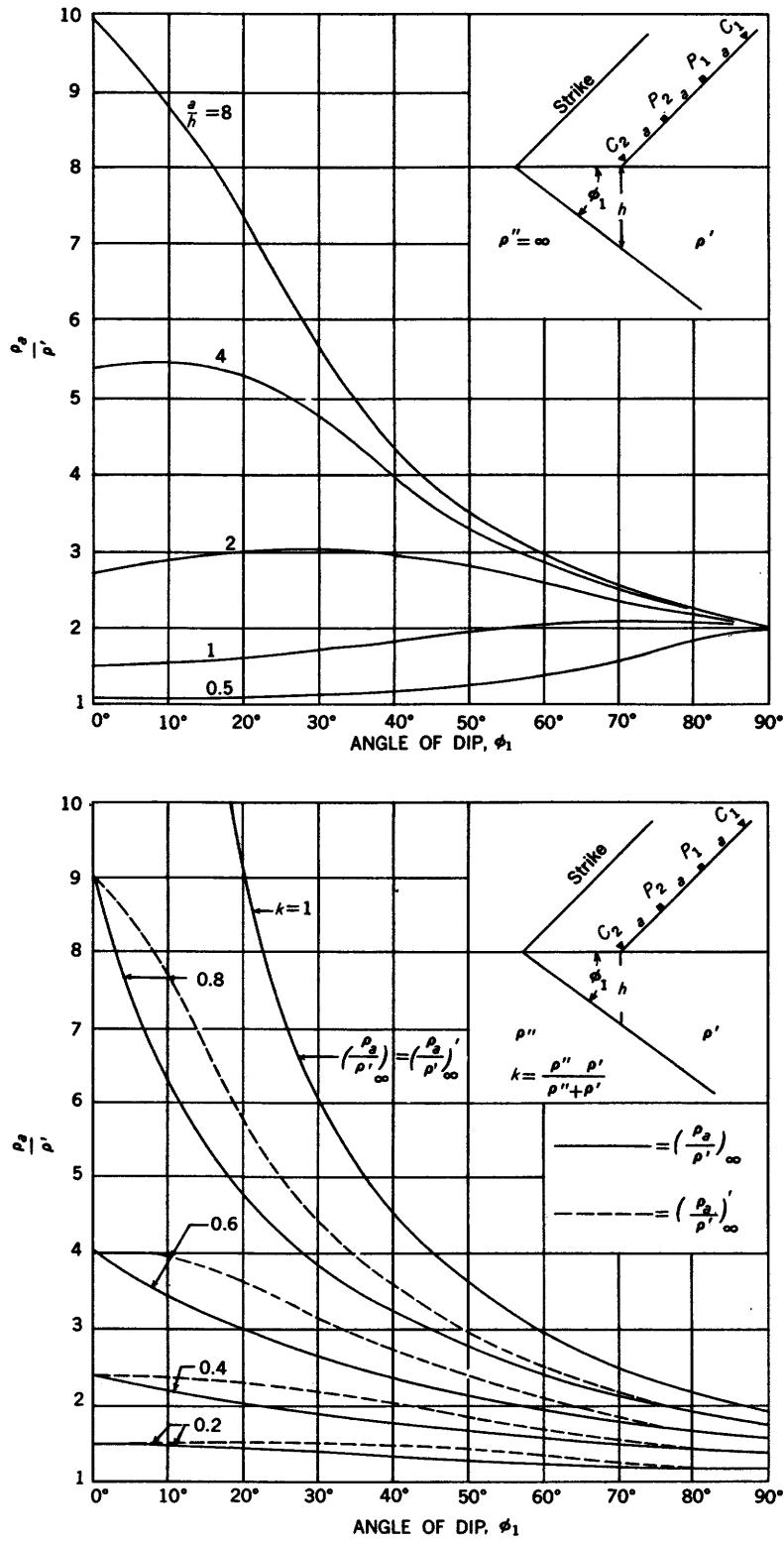
FIGURE 121.—Apparent-resistivity values for different angles of dip \phi_1 for vertical resistivity profiles over upper bed along traverse parallel to strike of dipping bed, Wenner configuration. Upper, Values for reflection factor k=+1 for various electrode separations. Adapted from Unz (1953). Lower, Asymptotic value for positive values of reflection factor k . Solid curves are exact values; dashed curves are values as obtained from image theory. Adapted from Unz (1953).
