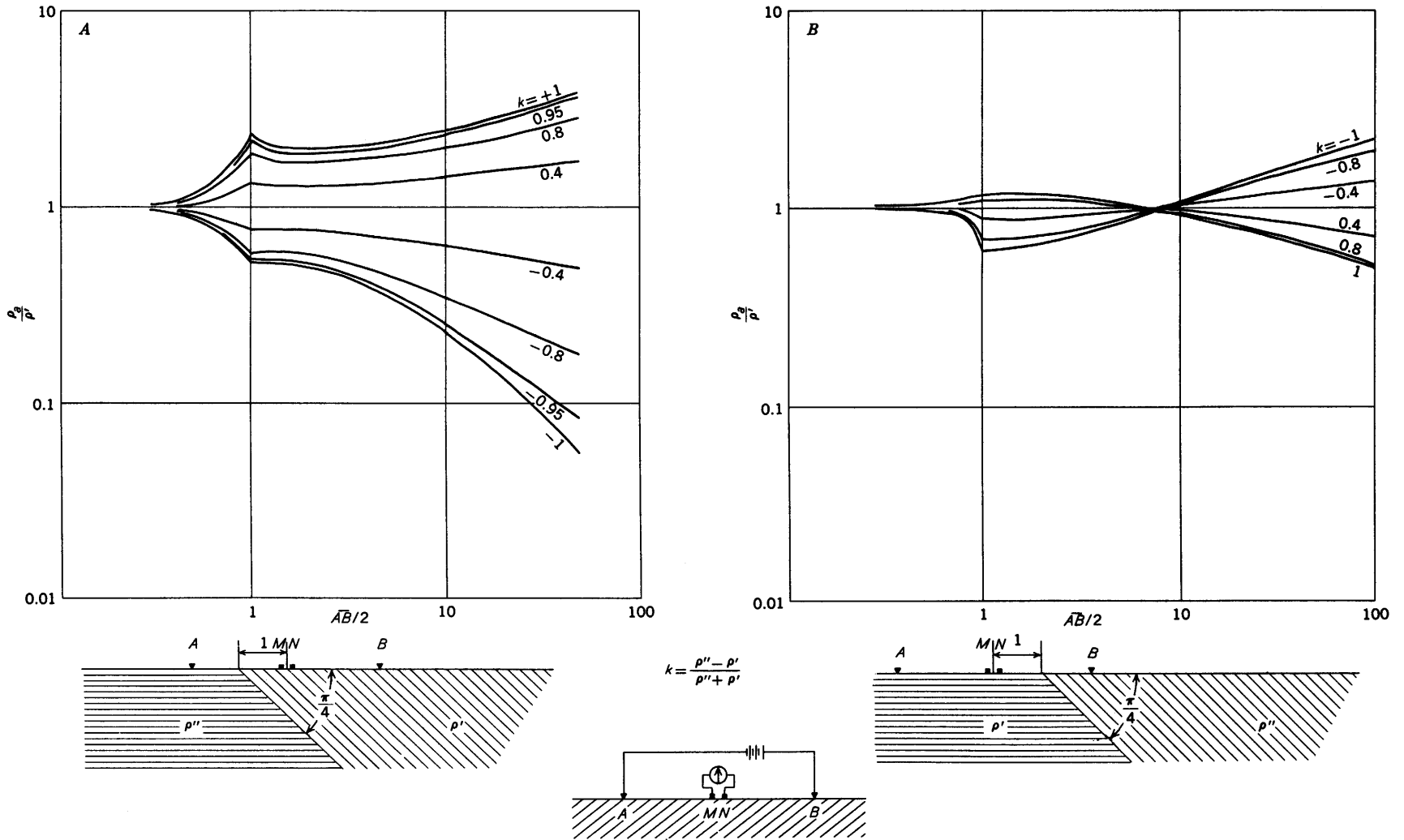
FIGURE 129.—Vertical resistivity profiles with Schlumberger configuration along traverse perpendicular to strike of bed dipping 45°. Profiles cross contact. Various values of reflection factor k . Adapted from Chastenet de Géry and Kunetz (1956).
