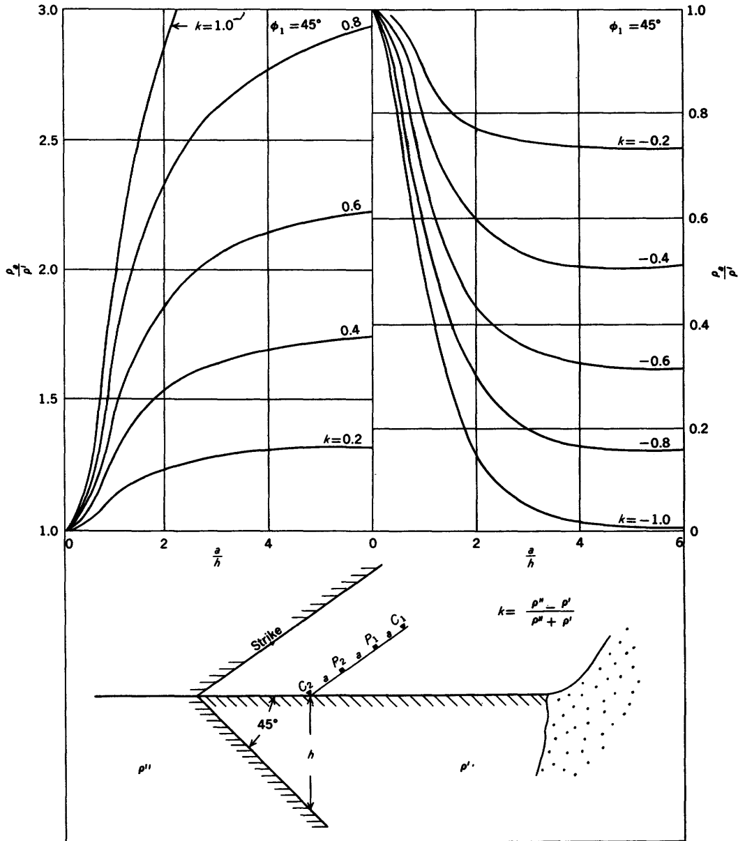
FIGURE 125.—Vertical resistivity profiles over upper bed along traverses parallel to strike of bed dipping 45°, Wenner configuration. Reflection factor k = \pm 1.0, \pm 0.8, \pm 0.6, \pm 0.4, and \pm 0.2 . Adapted from Maeda, 1955.
