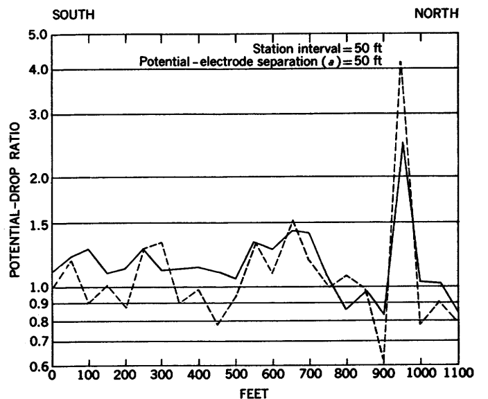
FIGURE 107.—Profile with constant-spacing system of potential-drop-ratio method across graphite zone, Graphite mine, Port Lincoln, South Australia. PDR data are not normalized. Adapted from Broughton Edge and Laby (1931).
