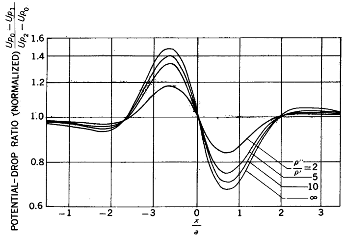
FIGURE 178.—Profiles with constant-spacing system of potential-drop-ratio method across buried spheres of different finite resistivity contrasts with surrounding country rock; spheres more conducting than country rock. Data are normalized. For all curves, c=10 ; d=1.25r_1=1.25a ; a =unity. Adapted from Kiyono (1950c) by permission of Kyōtō University.
