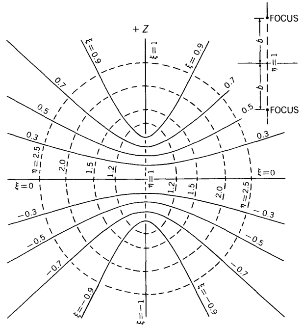
FIGURE 25.—Prolate spheroidal coordinates. Surfaces of constant third dimension are azimuthal planes through the vertical z -axis.
