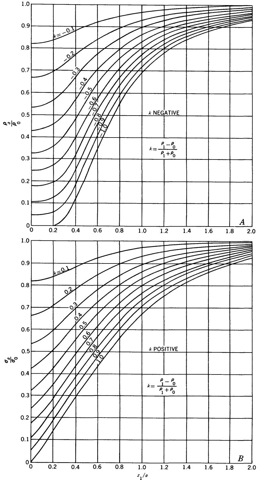
FIGURE 35.—(A) Apparent-resistivity (B) apparent-conductivity curves for Tagg interpretation of two-layer case, linear plotting; reflection factor k , (A) negative; and (B) positive. Adapted from Tagg (1932). Copyright by Am. Inst. Mining Metall. Engineers.
