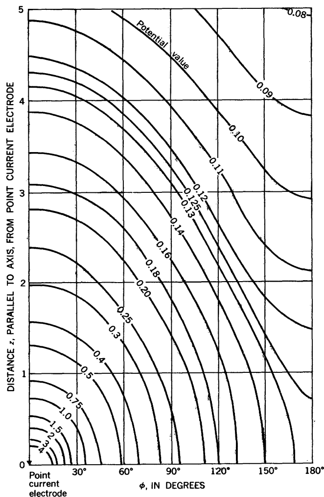
FIGURE 183.—Plot of the values of the actual potential at cylindrical coordinate points z and \phi on the surface of a perfectly insulating cylinder of infinite length due to point-current electrode C also on the surface of the cylinder at the origin z=0 ; \phi=0 ; radius of cylinder is unity. (See fig. 182.) Adapted from Huber (1953).
