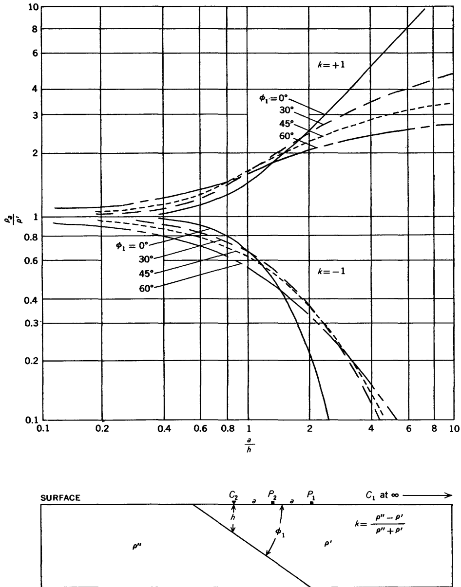
FIGURE 130.—Vertical resistivity profiles over upper bed along traverse perpendicular to strike of perfectly insulating (reflection factor k=+1 , upper set of curves) and conducting ( k=-1 , lower set of curves) lower beds dipping at various angles \phi_1 , asymmetrical Wenner configuration. Current electrode is closer to outcropping trace of contact than potential electrodes. Adapted from Maeda (1951b).
