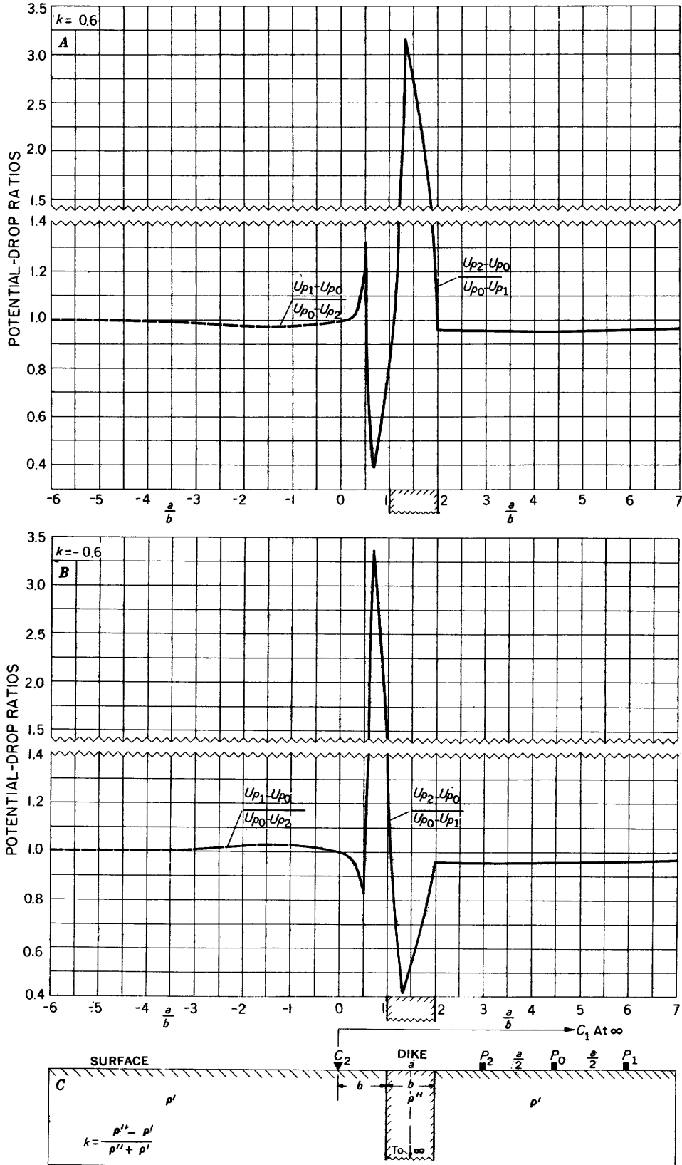
FIGURE 111.—Profiles with expanding-electrode system of potential-drop-ratio method across a vertical dike of width b , with current electrode C_2 at a fixed distance b from the dike. Data are normalized. Reflection factors are (A) k = +0.6 ; (B) k = -0.6 .
