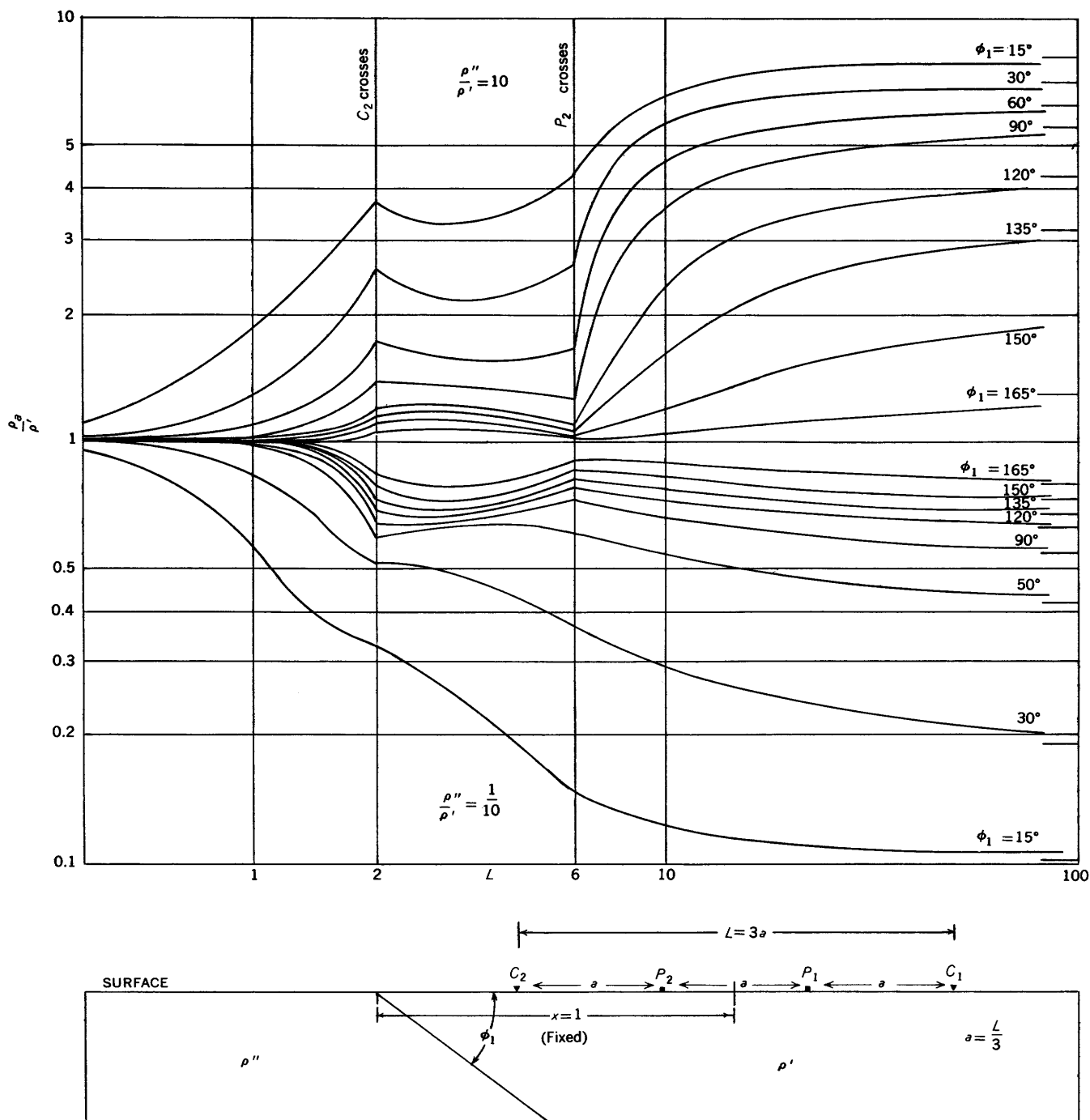
FIGURE 138.—Vertical resistivity profiles along traverse perpendicular to strike of beds of finite-resistivity contrasts ( \rho''/\rho' = 10 and \rho''/\rho' = 1/10 ) and dipping at various angles \phi_1 , Wenner configuration. Profiles across contact. d = 1 unit. Adapted from Huber (1955) by permission of Springer-Verlag, Vienna, Austria.
