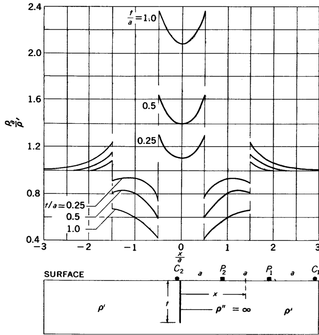
FIGURE 164.—Horizontal resistivity profiles across outcropping perfectly insulating thin vertical plates of different depths t , Wenner configuration (two-dimensional approximation); a =unity. Adapted from Kiyono (1950c) by permission of Kyōtō University.
