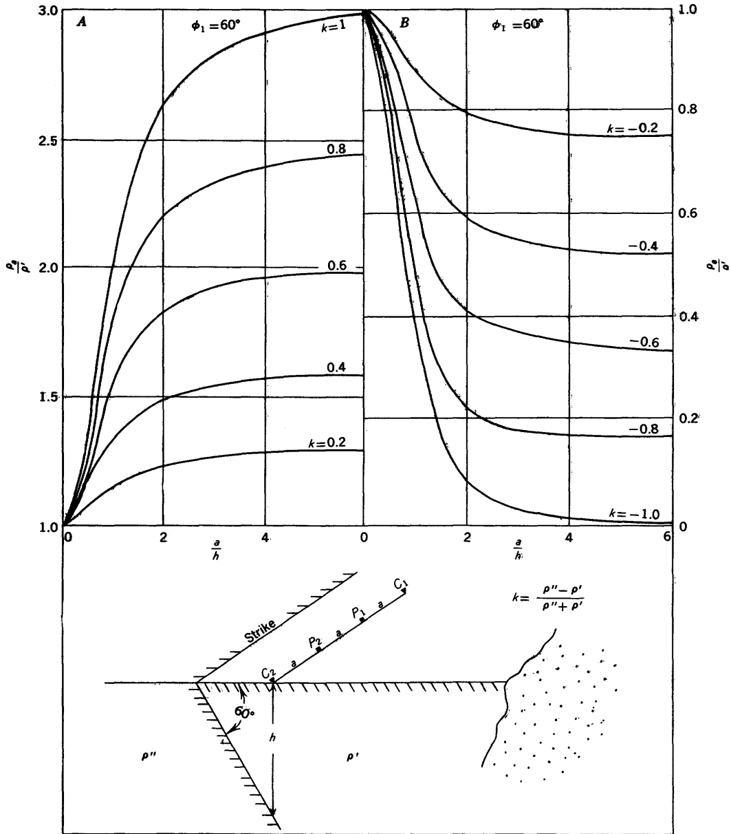
FIGURE 126.—Vertical resistivity profiles over upper bed along traverses parallel to strike of bed dipping 60°, Wenner configuration. Reflection factor k = \pm 1.0, \pm 0.8, \pm 0.6, \pm 0.4, \text{ and } \pm 0.2 . Adapted from Maeda (1955).
