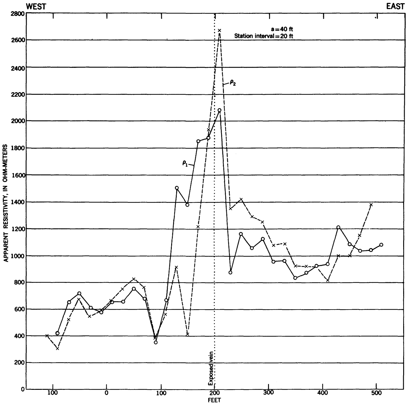
FIGURE 92.—Horizontal resistivity profile across exposed Sneed 1-B quartz vein, Vance County, N.C., Lee configuration (offset plotting). Electrode separation a=40 ft; station interval = 20 ft. G. R. MacCarthy and R. M. Shuler (1948, unpublished data).
