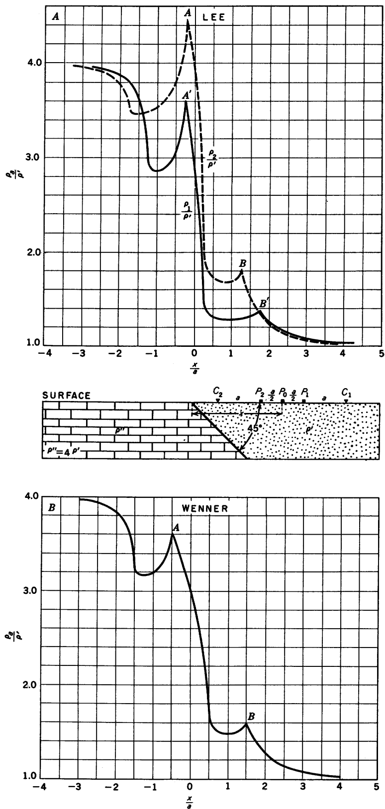
FIGURE 135.—Horizontal resistivity profiles with both the (A) Lee and (B) Wenner configurations along traverse perpendicular to strike of fault dipping 45^\circ . Profiles cross contact. Reflection factor k=+0.6 .
