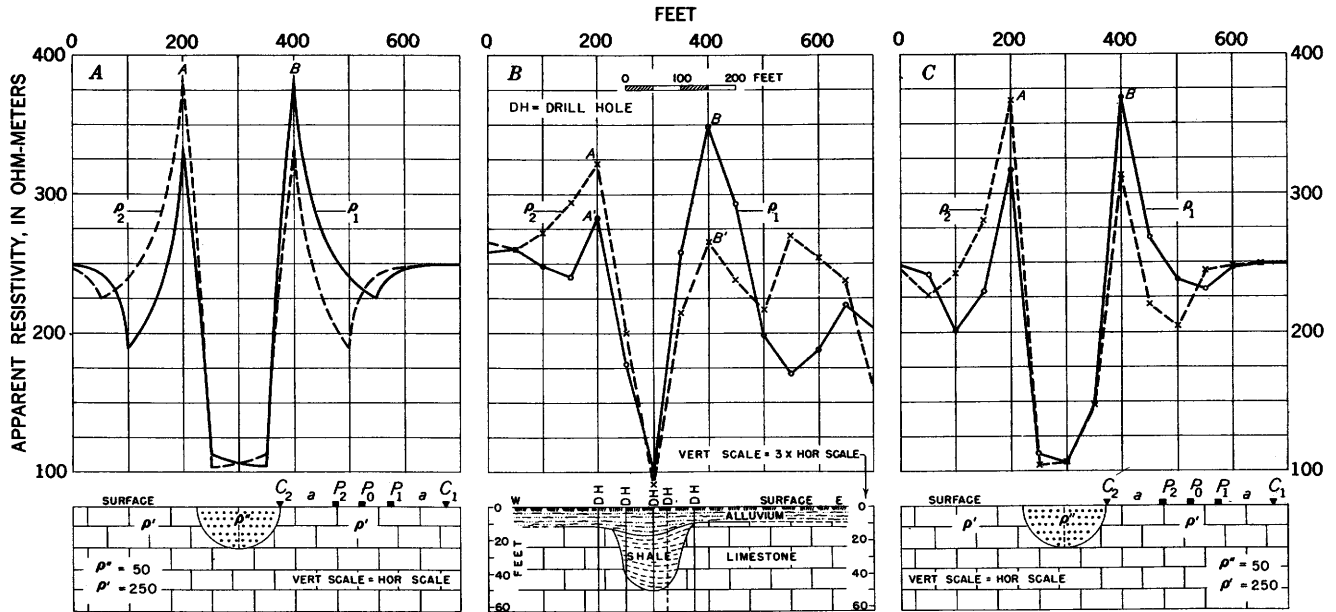
FIGURE 145.—Comparison of theoretical and observed horizontal resistivity profiles over filled sink, Lee configuration (offset plotting). (A) Continuous theoretical curve over hemispherical sink. (B) Observed field curve with geologic cross section. (C) Theoretical field plot over hemispherical sink. Assumed diameter of sink = 3a/2 . Assumed \rho''/\rho' = 50/250 . Adapted from Cook and Van Nostrand (1954).
