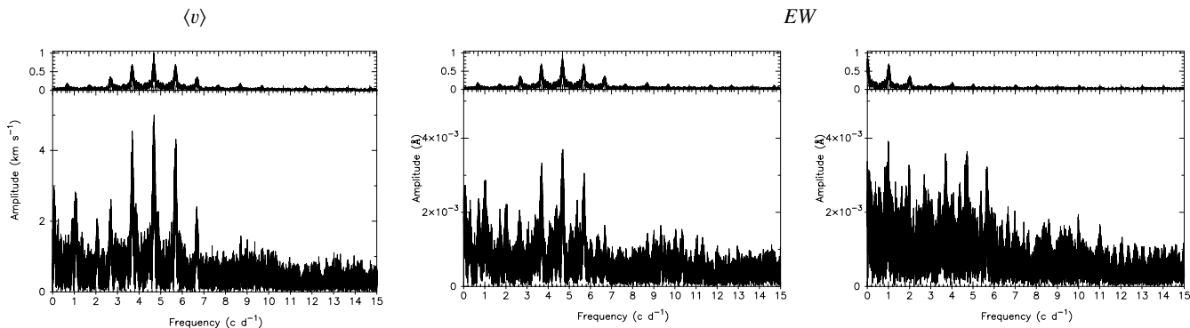
Fig. 2. Lomb-Scargle periodogram of the centroid radial velocity ( left ) and of the equivalent width ( middle and right ) derived from the profiles near 4552 Å ( left and middle ) and 4568 Å ( right ). On top of each figure the window function, shifted according to the highest peak in the periodogram, is given.
