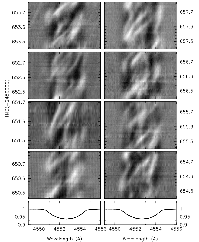
Fig. 1. Grayscale representations of the observed line profiles obtained during eight consecutive nights from 20–28 July 1997. The residual Si III 4552.654 Å profiles with respect to the average profile of the eight nights are plotted in a shade of gray: black represents a positive residual while white represents a negative residual. Bottom: the average profile of the eight nights.
