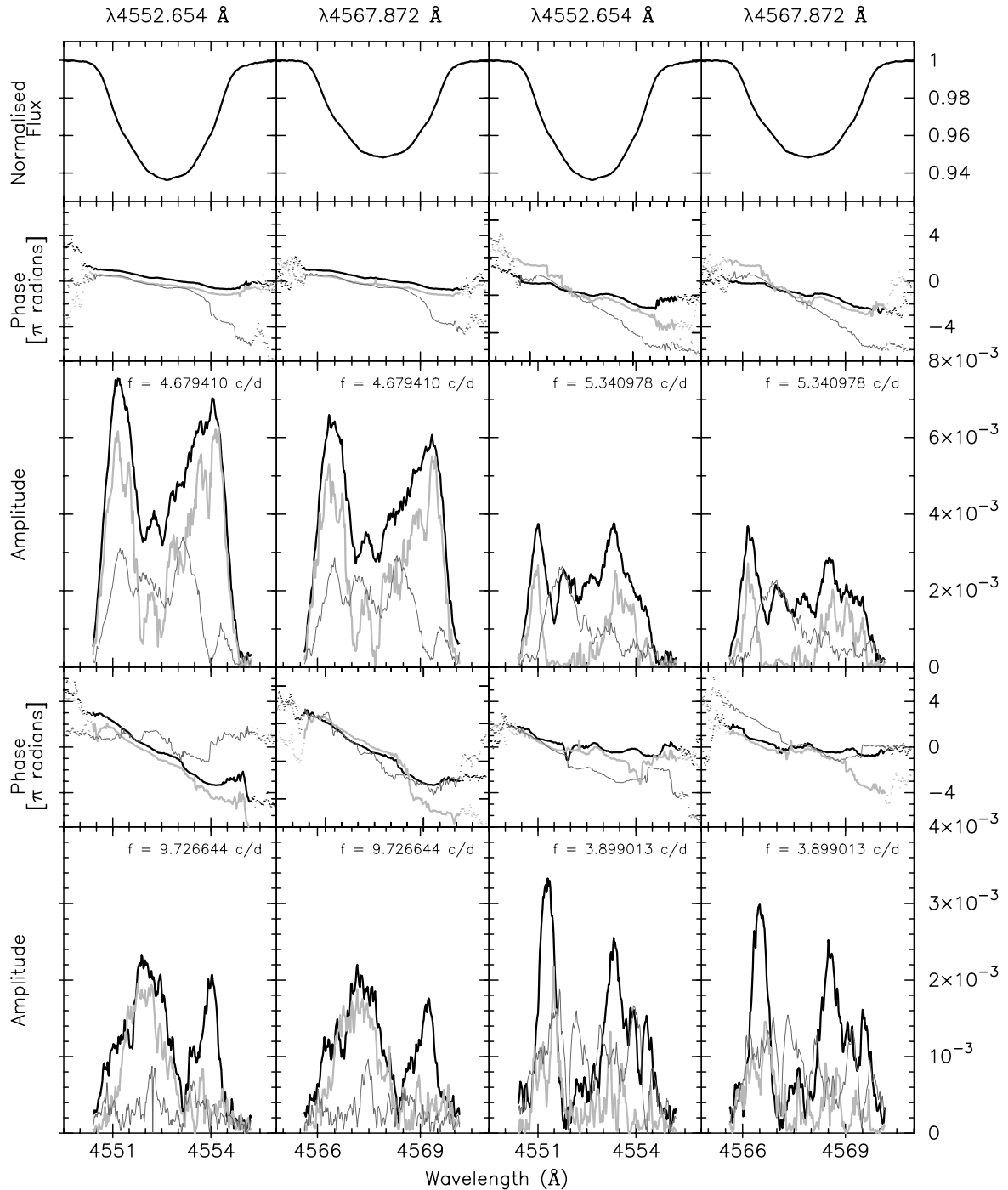
Fig. 8. Mean profile and IPS diagrams for the variability in the 4552.654 Å and 4567.872 Å line profile at f_i and its first harmonic, with f_i indicated in the panels: f_1 (top panels, left); f_3 (top panels, right), f_4 (bottom panels, left), and f_2 (bottom panels, right). The phase diagrams (middle of each panel) are expressed in \pi radians. The amplitude diagrams (bottom of each panel) give the amplitude of the variations of respectively f_i and 2f_i in the line profiles expressed in units of normalised flux. Thick black line: single-sinusoid fit f_i ; light gray line: CLEANed Fourier transform f_i ; thin black line: single-sinusoid fit 2f_i . Note the difference in scale of the amplitude diagrams in the upper and lower panels.
