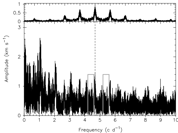
Fig. 6. Lomb-Scargle periodogram for \langle v \rangle calculated from the 4552.654 Å profile after prewhitening with all frequencies listed in Table 3. The dashed line is drawn at the position of f_1 = 4.679410 c d -1 and shows that frequencies very close to f_1 are still present in the residuals of \langle v \rangle . The gray boxes mark the frequency regions that were used to determine the noise level.
