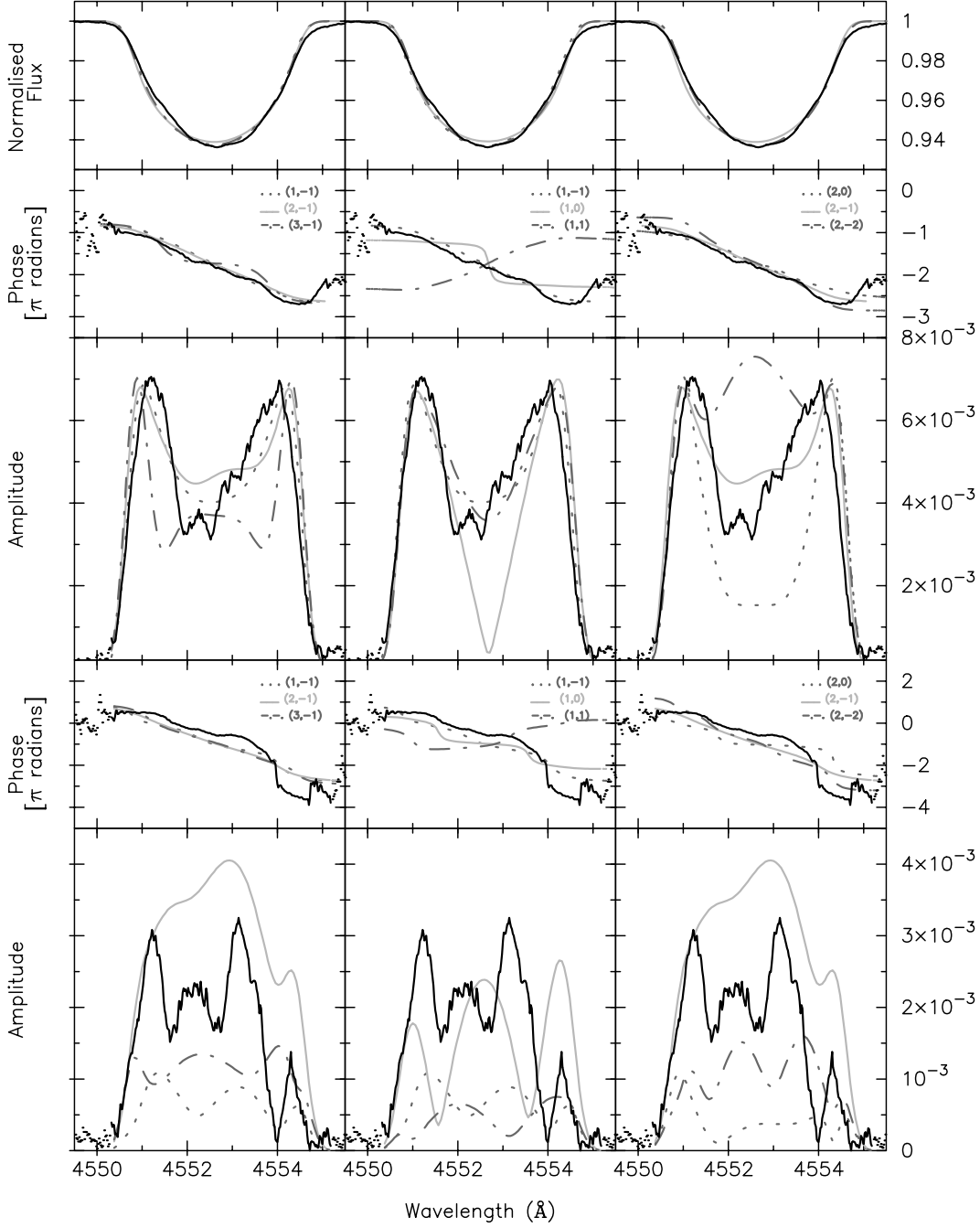
Fig. 9. Mean profile, phase and amplitude diagrams of frequency f_1 (top) and 2f_1 (bottom) in the wavelength region of the 4552.654 Å line, as calculated from single-sinusoid fits. The solid black line represents the diagnostics derived from the observed data. The other lines are derived from theoretically calculated profiles with parameters: v \sin i = 125 \text{ km s}^{-1} , i = 80^\circ , \sigma = 18.75 \text{ km s}^{-1} , dT/T = 0.03 and k = 0.20 . Left panel: m = -1 and different values of l : l = 1 (dotted dark gray line), l = 2 (solid light gray line) or l = 3 (dashed-dotted dark gray line). Middle panel: l = 1 and different values of m : m = -1 (dotted dark gray line), m = 0 (solid light gray line) or m = 1 (dashed-dotted dark gray line). Right panel: l = 2 and different values of m : m = 0 (dotted dark gray line), m = -2 (solid light gray line) or m = -1 (dashed-dotted dark gray line). The phases are given in \pi radians; the amplitudes are expressed in terms of normalised flux of the line profile.
