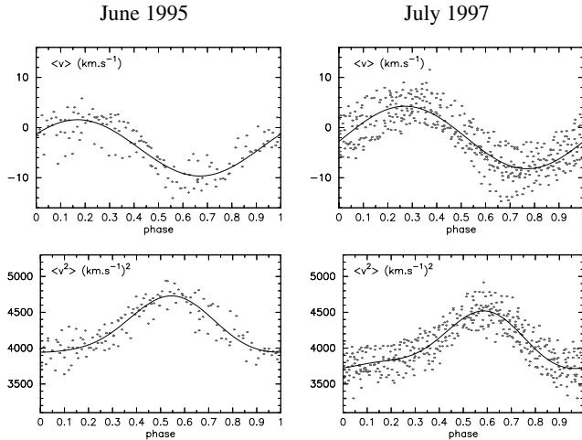
Fig. 5. \langle v \rangle and \langle v^2 \rangle calculated from the 4552.674 Å profiles of June 1995 and July 1997 fitted and folded with f_1 = 4.679410 c d -1 (top) and fitted with f_1 and 2f_1 (bottom). The dots are the observations while the full line is the least-squares fit. The amplitudes of the variations in \langle v \rangle and \langle v^2 \rangle calculated from the dataset of June 1995 are significantly different from the corresponding amplitudes calculated from the dataset of July 1997, as shown in Table 1.
