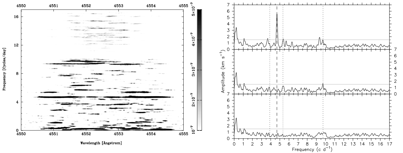
Fig. 7. Power spectrum ( left ) and summed periodogram across the line profile ( right ) of the Si III line at 4552.654 Å of \lambda Scorpii, obtained by an IPS analysis. For each wavelength bin the power as a function of frequency is coded in gray. Left : power spectrum of the data. The main peak occurs at the frequency f_1 . Right : summed periodograms of the original data, of the data after prewhitening with f_1 and its first harmonic and of the data after prewhitening with all the frequencies listed in Table 3 and their first harmonic. The horizontal light gray line shows the 4 S/N level. f_1 is indicated by a dashed line while the positions of f_2 , f_3 and f_4 are marked by a dotted line.
