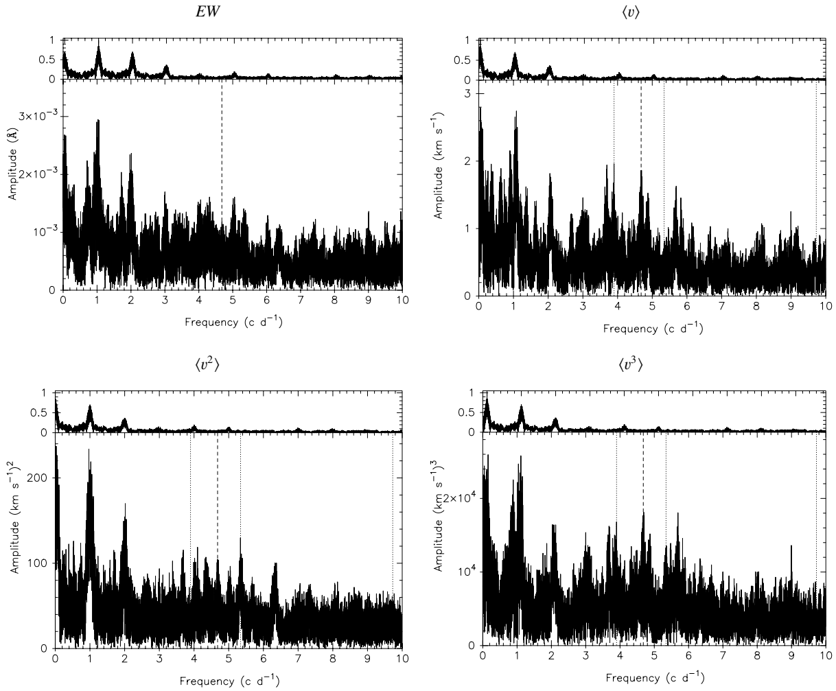
Fig. 4. Lomb-Scargle periodograms of the residuals of the equivalent width and of the first three velocity moments calculated from the 4552.654 Å profiles after prewhitening with frequency f_1 = 4.679410 c d ^{-1} and its first harmonic. A frequency similar to f_1 (dashed line) is still present in the variability of the moments. Candidate additional frequencies f_2 = 3.899013 c d ^{-1} , f_3 = 5.340978 c d ^{-1} and f_4 = 9.726644 c d ^{-1} are indicated by dotted lines. On top of each figure the window function, shifted according to the highest peak in the periodogram, is given.
