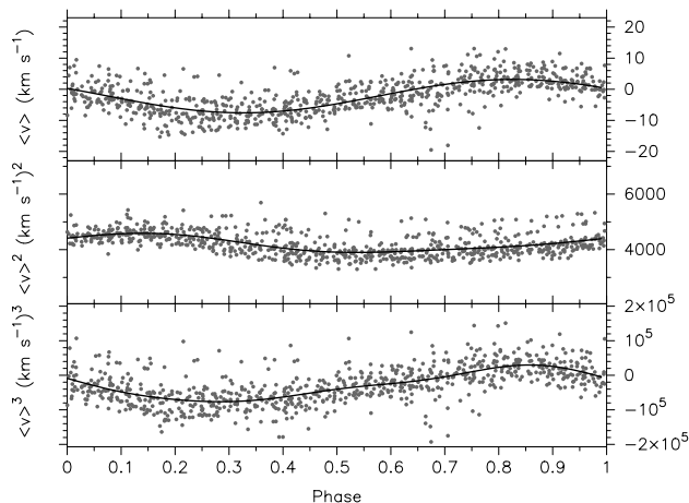
Fig. 3. The first three normalised moments of the Si III 4552.654 Å line of \lambda Scorpii folded with f_1 = 4.679410 c d -1 . The three fits take respectively f_1 ; f_1 and 2f_1 ; f_1 , 2f_1 and 3f_1 into account.
