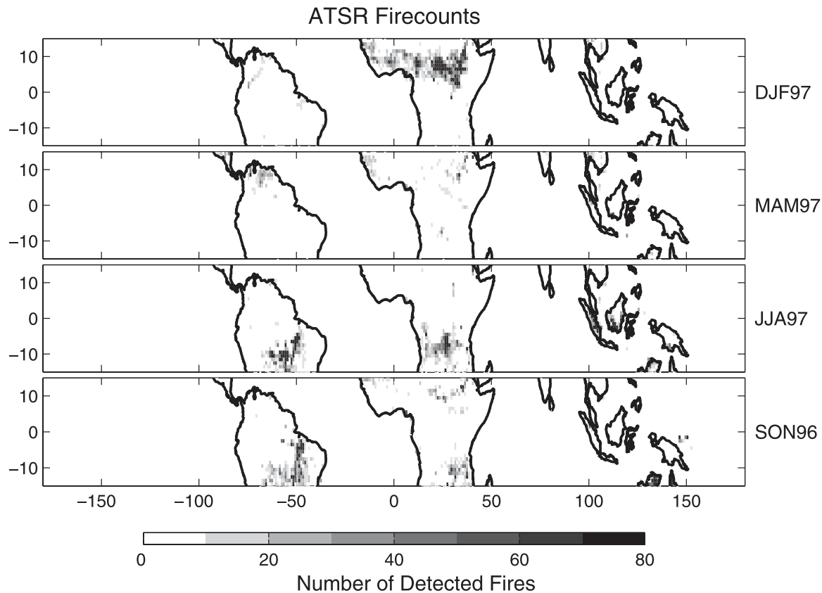
Figure 1. Seasonally averaged fire-counts from the Along Track Scanning Radiometer for December 1996–February 1997 (DJF97), March 1997–May 1997 (MAM97), June 1997–August 1997 (JJA97), and September 1996–November 1996 (SON96). Data are from Arino and Rosaz [1999].
