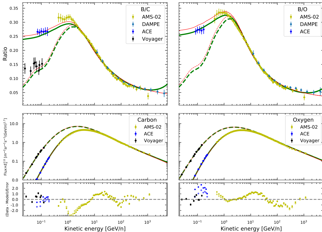
FIG. 6: B/C and B/O ratios (top panels), and C, O fluxes (bottom panels) for the models with secondary production (model F; red thin lines) and acceleration (model G; green thick lines) at source. Dashed lines are the spectra in the local ISM, and solid lines are modulated spectra near the Earth. Sub-panels of bottom ones show the residuals of the model fittings to the C and O spectra. The filled symbols are for model F and open symbols are for model G.
