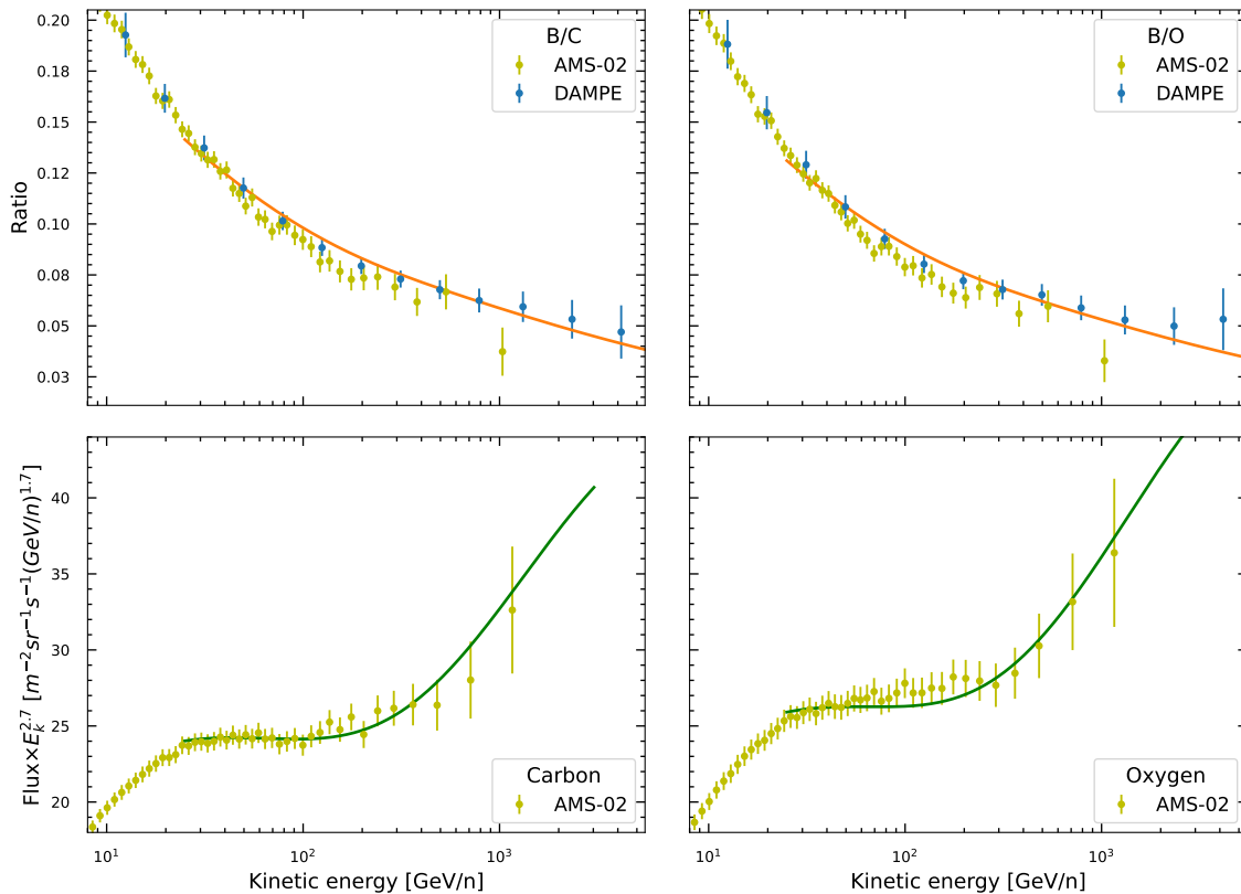
FIG. 3: B/C and B/O ratios (top panels), and C, O fluxes (bottom panels) for the model with re-acceleration by a nearby source.
