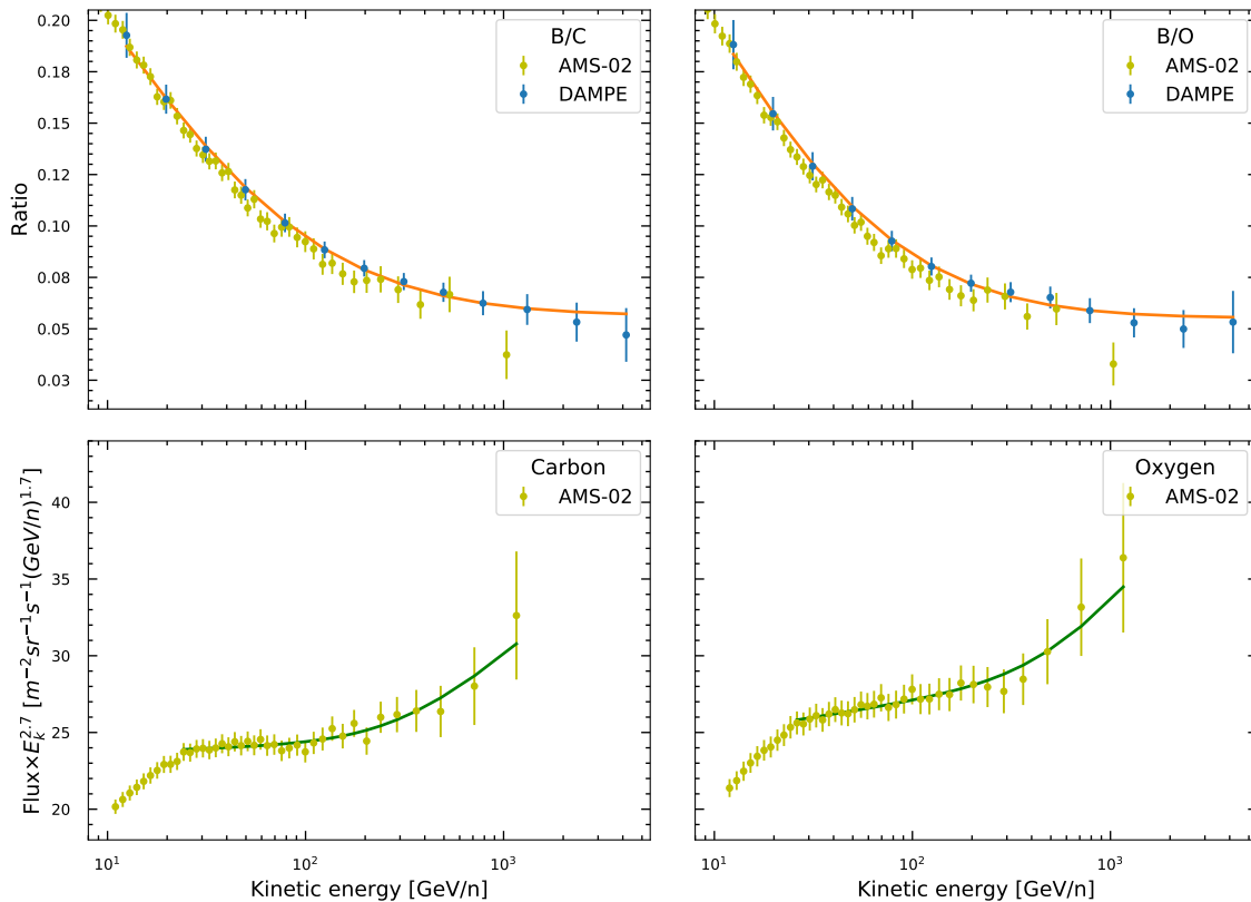
FIG. 1: B/C and B/O ratios (top panels), and C, O fluxes (bottom panels) for the NLB model.
