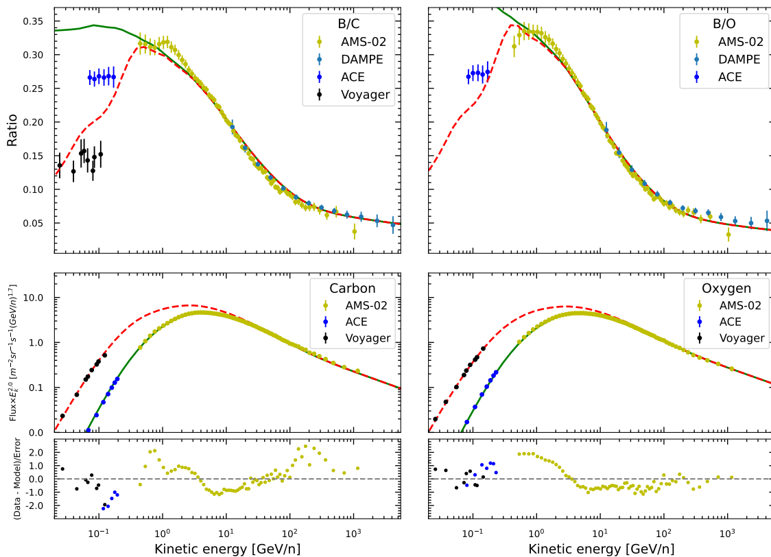
FIG. 5: B/C and B/O ratios (top panels), and C, O fluxes (bottom panels) for the Self-generated turbulence model. Dashed lines are the spectra in the local ISM, and solid lines are modulated spectra near the Earth. Sub-panels of bottom ones show the residuals of the model fittings to the C and O spectra.
