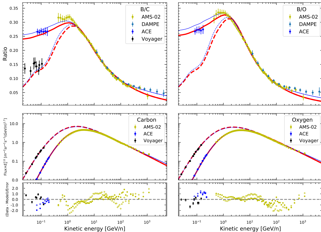
FIG. 2: B/C and B/O ratios (top panels), and C, O fluxes (bottom panels) for the re-acceleration model. Red thick lines show the results for the diffusion coefficient of Eq. (2), and blue thin lines show the results for the diffusion coefficient with an additional high-energy break. Dashed lines are the spectra in the local ISM, and solid lines are modulated spectra near the Earth. Sub-panels of bottom ones show the residuals of the model fittings to the C and O spectra. The open symbols are for model B and filled symbols are for model B’.
