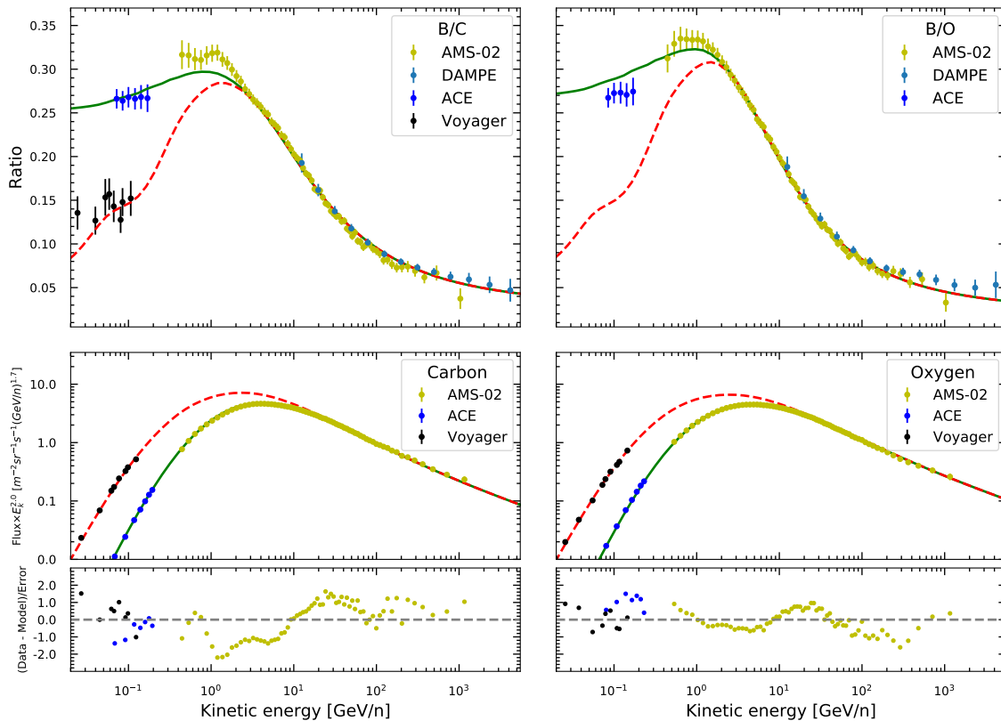
FIG. 4: B/C and B/O ratios (top panels), and C, O fluxes (bottom panels) for the spatially-dependent propagation model. Dashed lines are the spectra in the local ISM, and solid lines are modulated spectra near the Earth. Sub-panels of bottom ones show the residuals of the model fittings to the C and O spectra.
