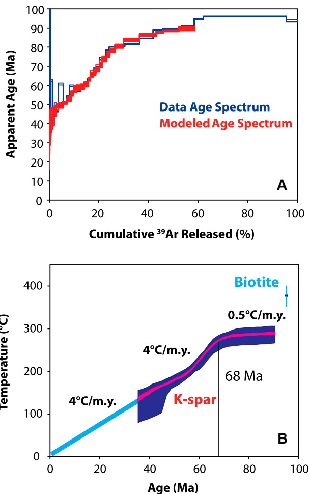
Figure 9. (A) Down-stepping K-feldspar ^{40}\text{Ar}/^{39}\text{Ar} age spectra (blue) from a granitoid sample (01KIM) in the Alaska Range along with modeled age spectra (red) produced using the software of Lovera et al. (2002) indicating a prolonged and complex thermal history. (B) Cooling history of sample 01K1 M from multidiffusion domain model (MDD) thermal models generated from K-feldspar and biotite ( 94.8 \pm 0.5 \text{ Ma} ) using the software of Lovera et al. (2002). The MDD magenta band is the 90% confidence interval of the mean, and the purple band is the 90% confidence of the distribution. The light blue line is a projection of the long-term cooling rate past the closure temperature of K-feldspar to the 0 \text{ }^{\circ}\text{C} intercept. The MDD thermal model from sample 01KIM demonstrates slow prolonged cooling starting at about 68 Ma at a long-term rate of approximately 6 \text{ }^{\circ}\text{C/m.y.} until around 52 Ma, when average cooling rate is slightly slower
